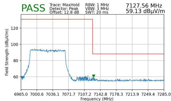
Plot 7-245. Radiated Upper Band Edge Plot MIMO (Peak – UNII Band 8 – 996T)
