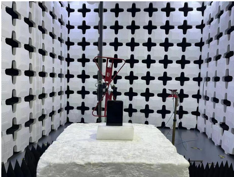
14. Radiated Emissions (Part 22/24/27,30MHz-18GHz)
