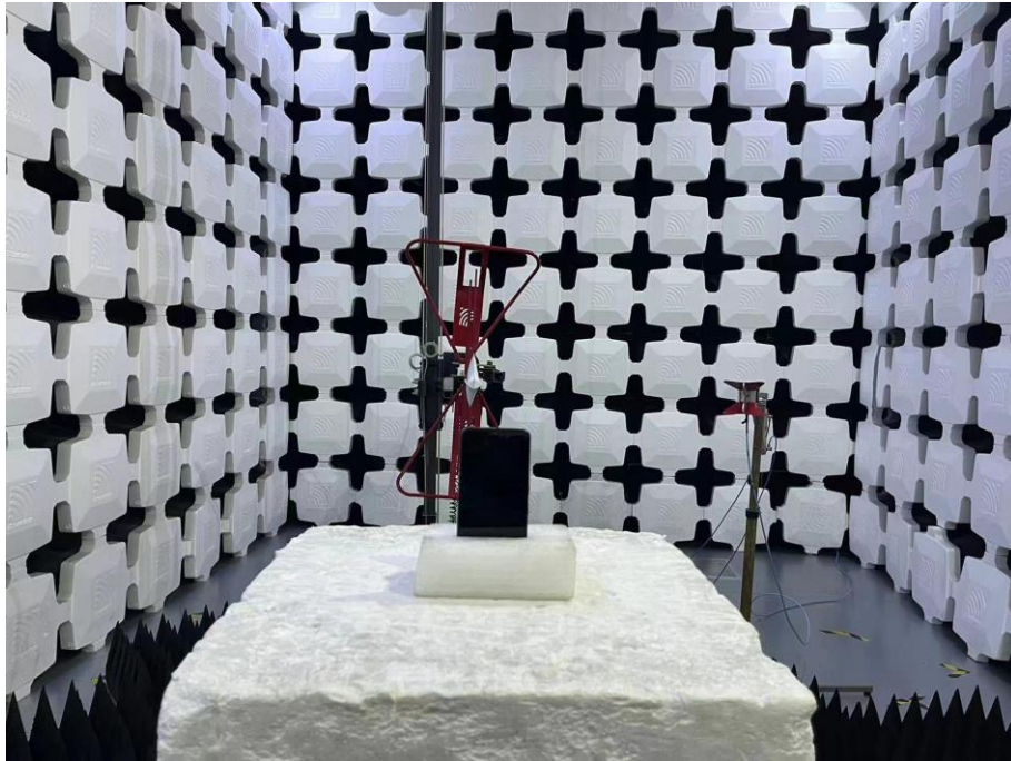
11. Radiated Emissions (Part 15C&Part 15E, 1GHz -18GHz)
