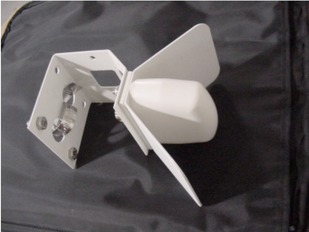
Figure 4: Mobile Mark 9dBi Corner Reflector
