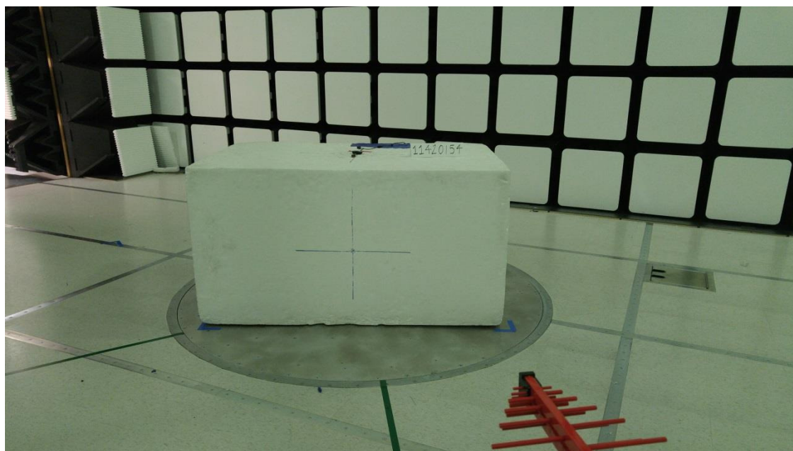
BELOW 1GHz PHOTO BACK
