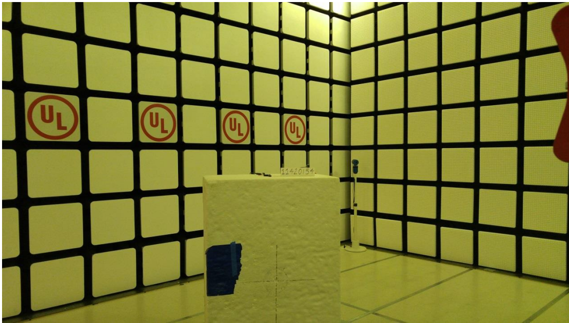
ABOVE 1GHz PHOTO FRONT
