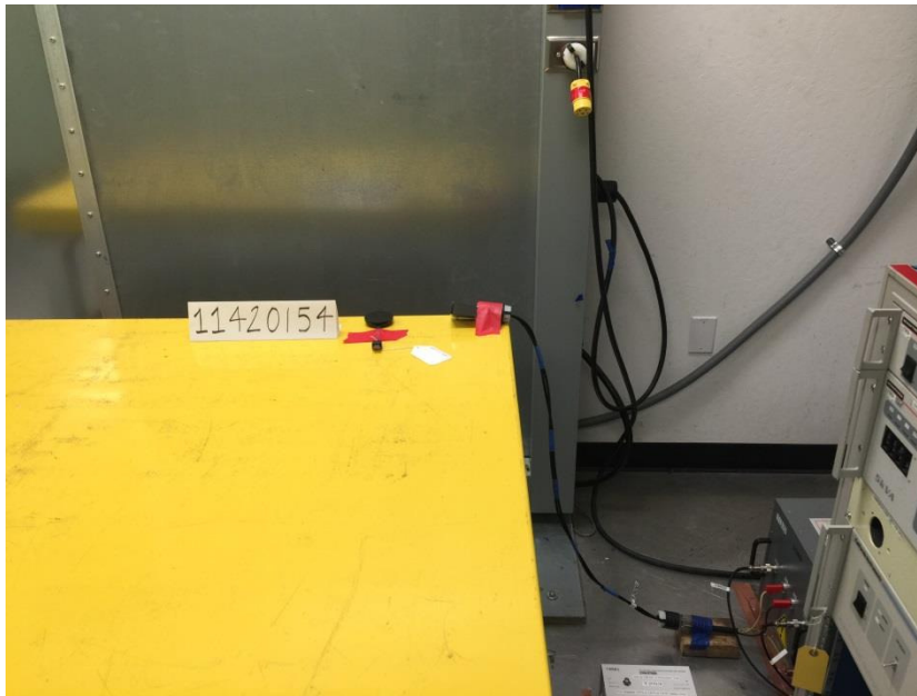
LINE CONDUCTED PHOTO FRONT
