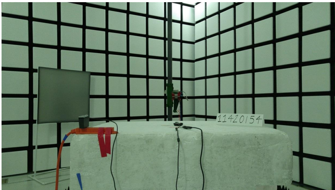
ABOVE 1GHz PHOTO BACK
