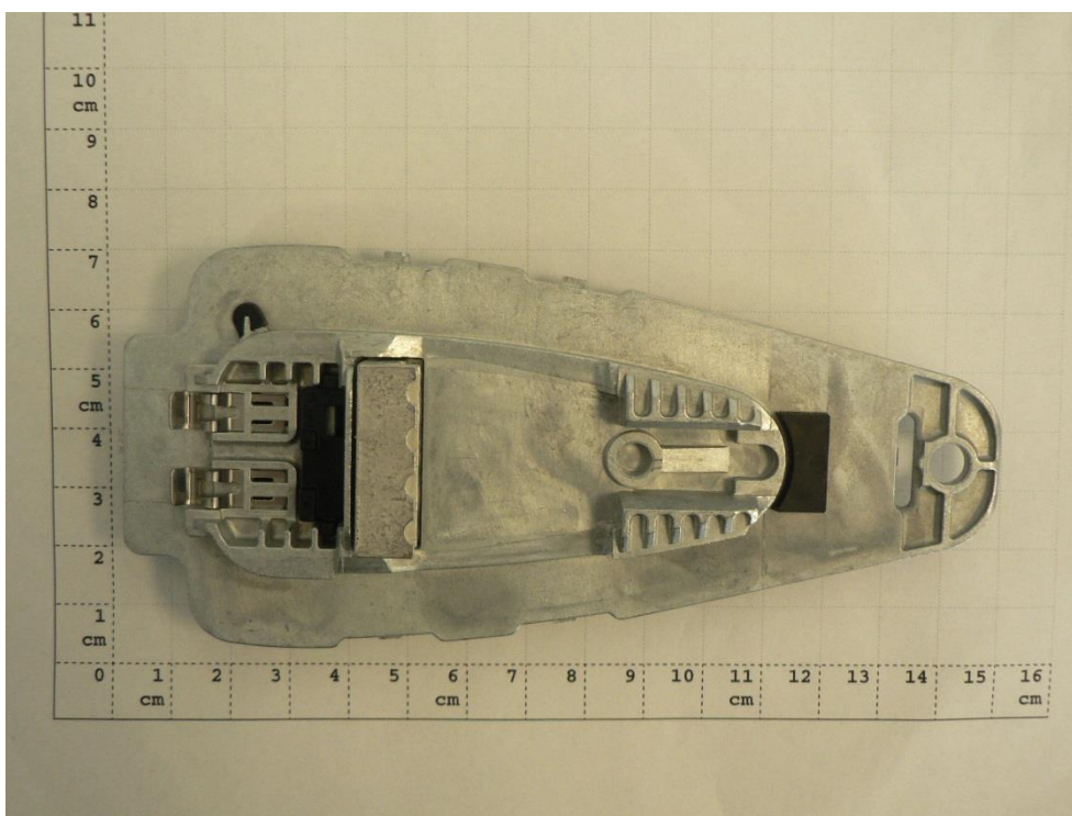
Photograph 9: Equipment under test: automotive roof pod base plate
