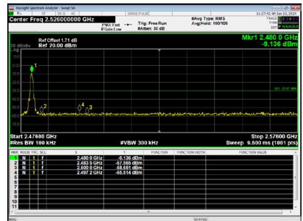
Band-edge Emission
