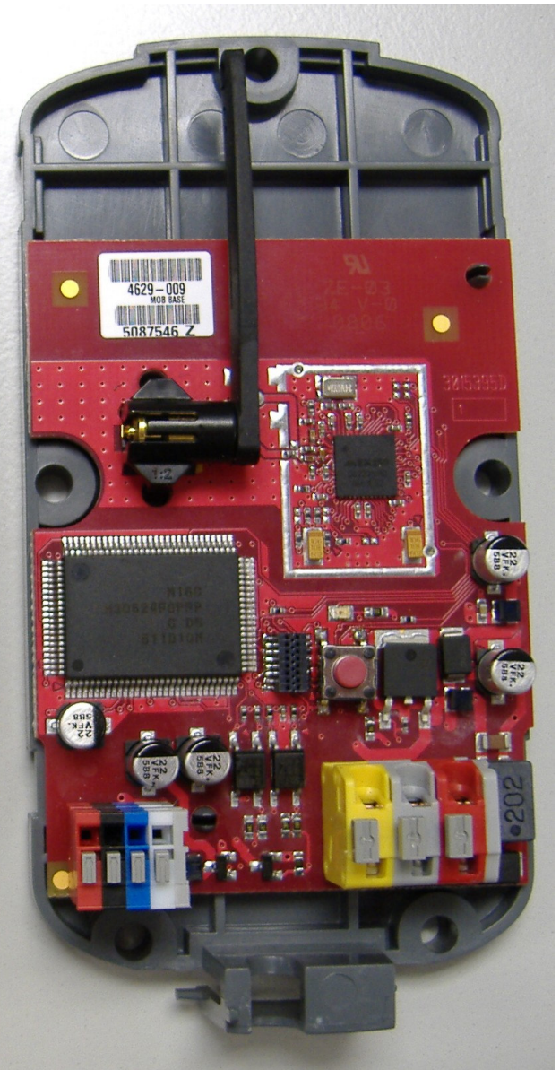
LT Base Station Front View, Primary and Secondary Covers Removed
