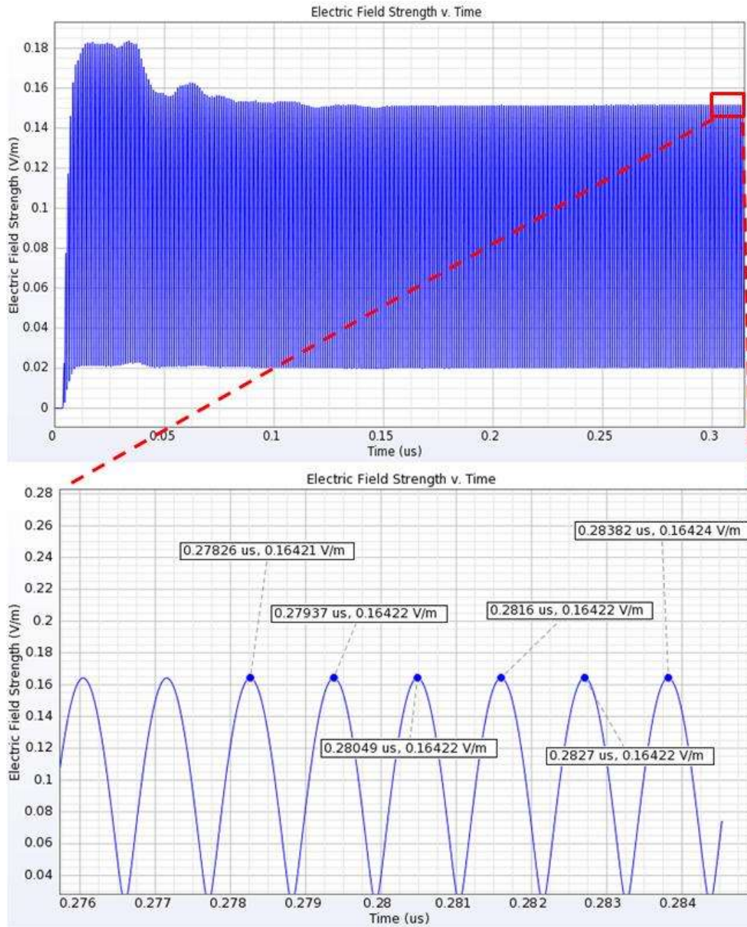
Sensor E-field strength vs. time used for the convergence analysis (bystander, 450 MHz).
