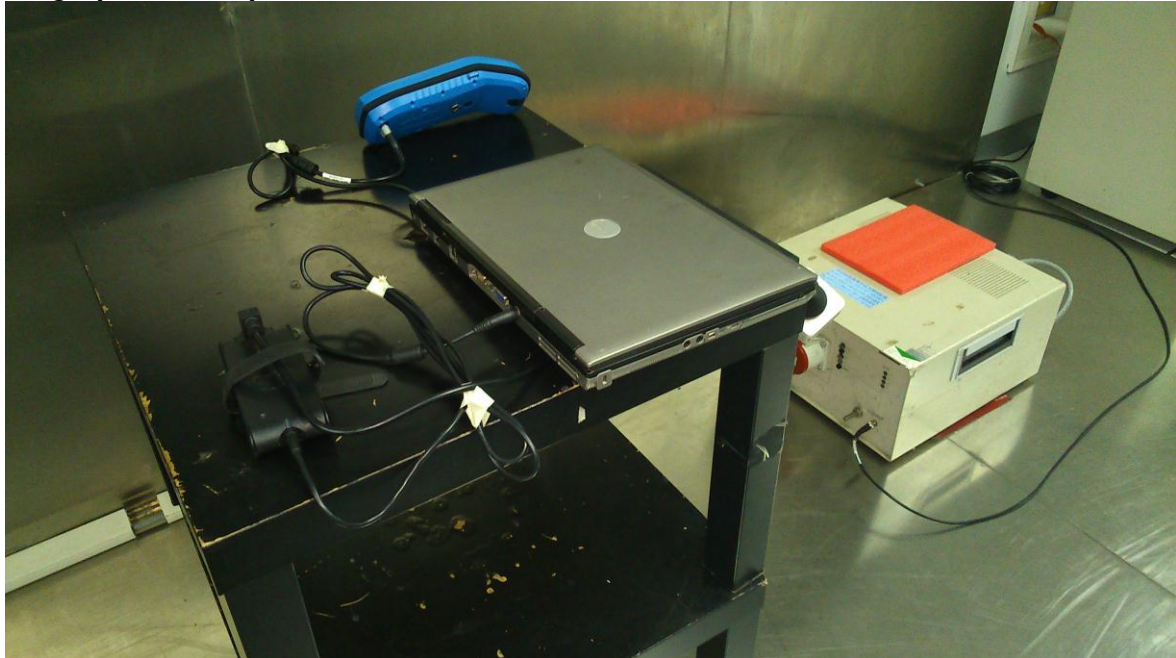
Photograph 2: Set-up for Radiated Emission of below 1GHz
