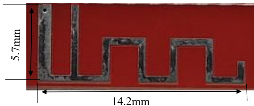
Antenna Photo & Length (mm)
