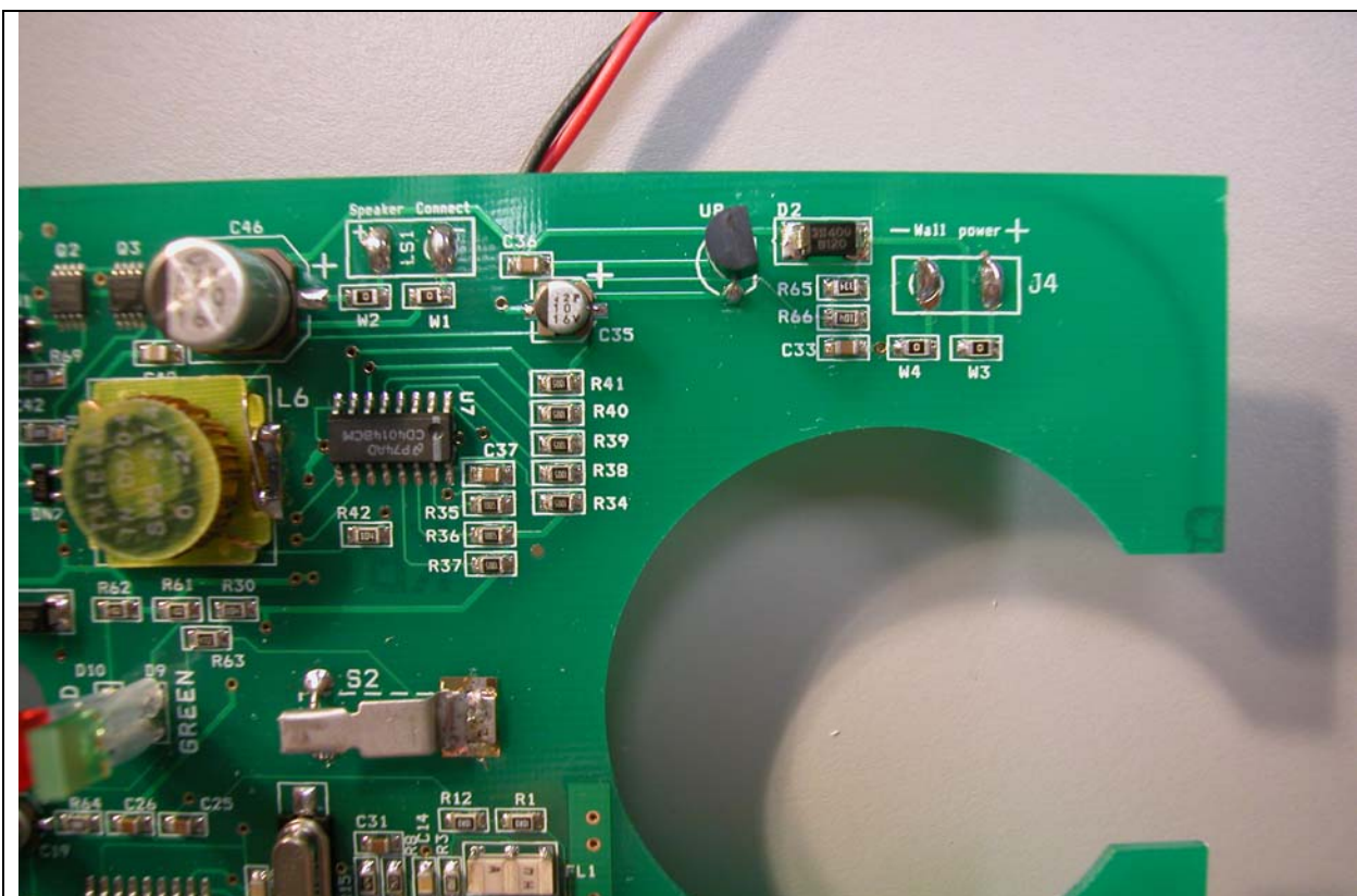
PCB front 2 Components
