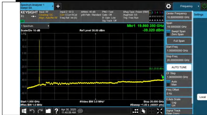
Band41-15MHz-QPSK-41515-1RB#74-1000~20000-PASS
