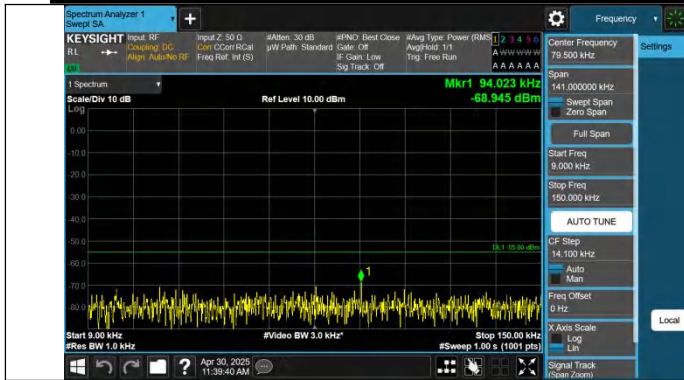
Band41-15MHz-QPSK-41515-1RB#0-0.009~0.15-PASS
