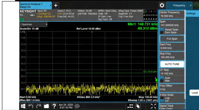
Band41-10MHz-QPSK-40620-1RB#0-0.009~0.15-PASS
