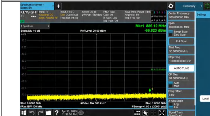
Band41-15MHz-QPSK-41515-1RB#0-30~1000-PASS
