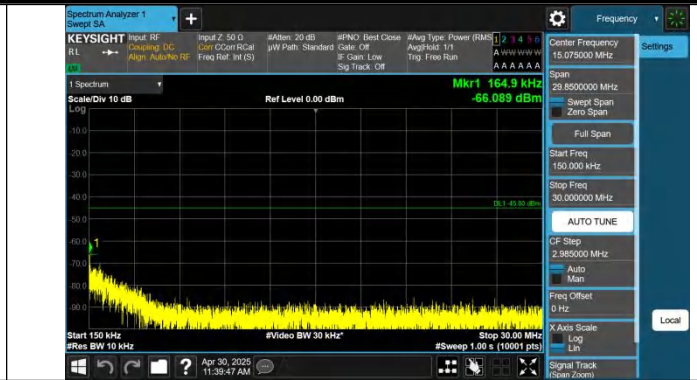
Band41-15MHz-QPSK-41515-1RB#0-0.15~30-PASS
