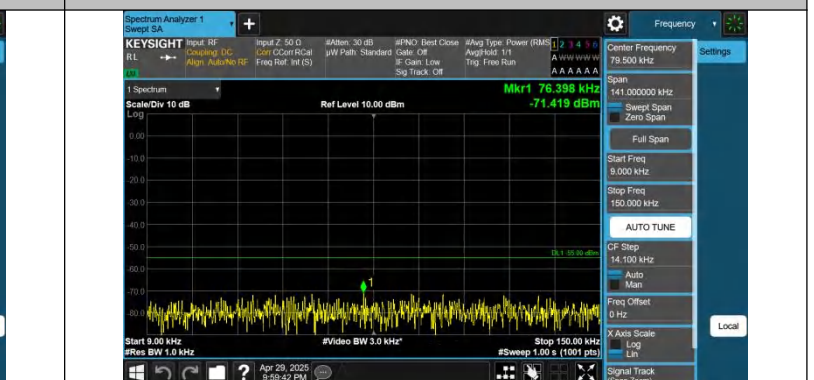
Band41-10MHz-QPSK-41540-1RB#49-0.009~0.15-PASS
