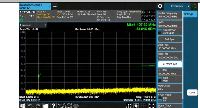
Band41-15MHz-QPSK-41515-1RB#74-30~1000-PASS
