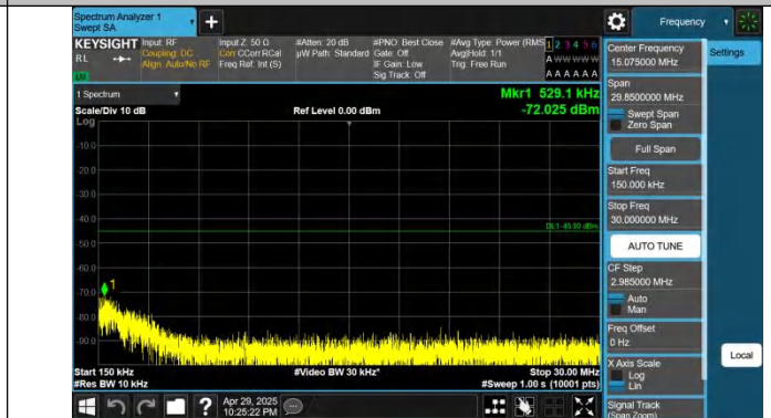
Band41-20MHz-QPSK-39750-1RB#0-0.15~30-PASS
