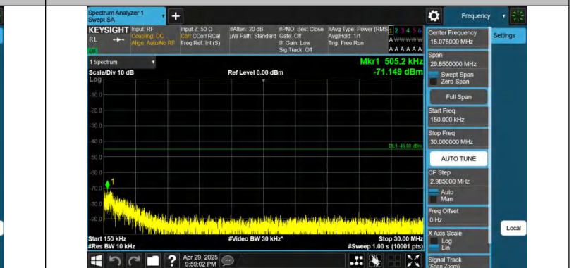
Band41-10MHz-QPSK-41540-1RB#0-0.15~30-PASS
