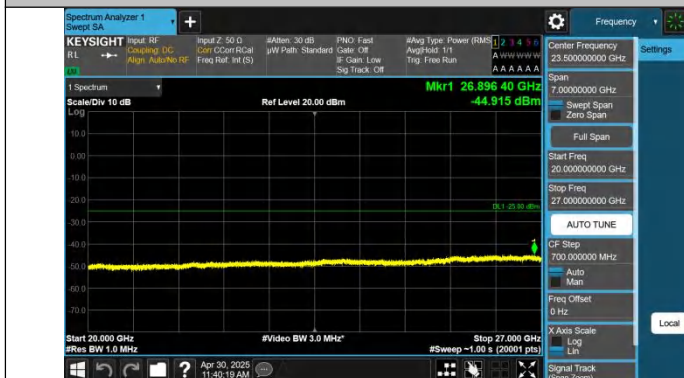
Band41-15MHz-QPSK-41515-1RB#0-20000~27000-PASS
