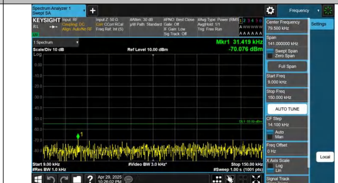
Band41-20MHz-QPSK-39750-1RB#99-0.009~0.15-PASS
