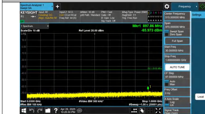
Band41-20MHz-QPSK-39750-1RB#0-30~1000-PASS
