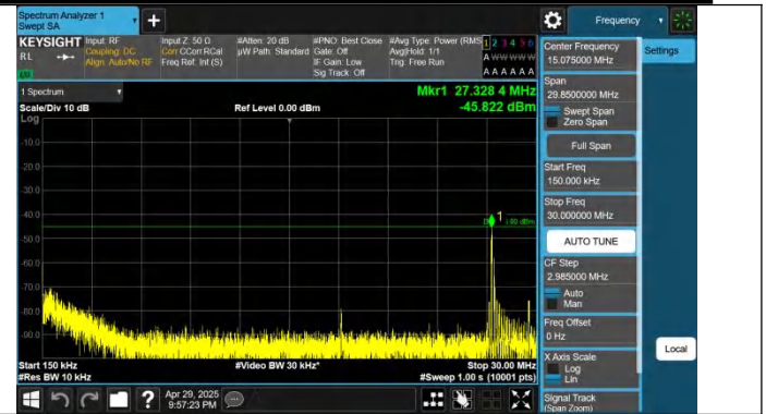
Band41-10MHz-QPSK-40620-1RB#0-0.15~30-PASS
