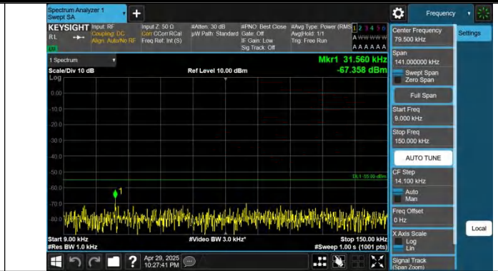
Band41-20MHz-QPSK-40620-1RB#99-0.009~0.15-PASS
