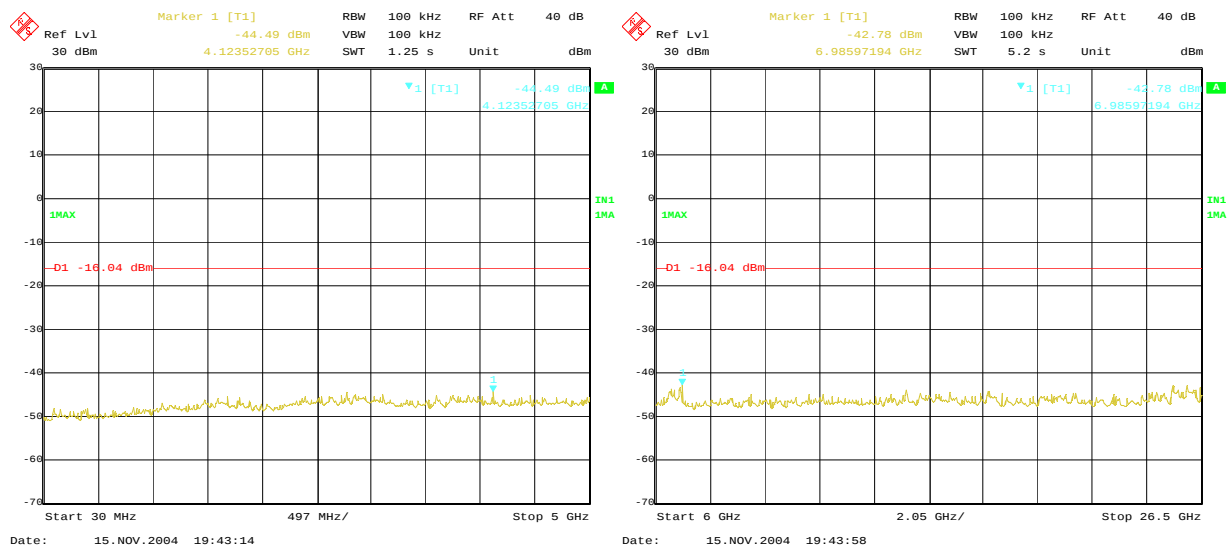
Plot 4-4-3. Out of band emissions around 5745MHz (OFDM, 6Mbps)
