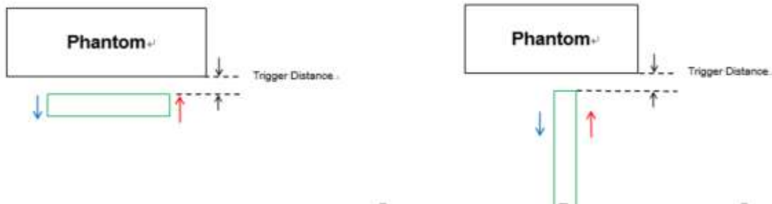
Proximity Sensor Trigger Distance Assessment KDB 616217 D04 §6.2 (Rear / Bottom / Right side)
