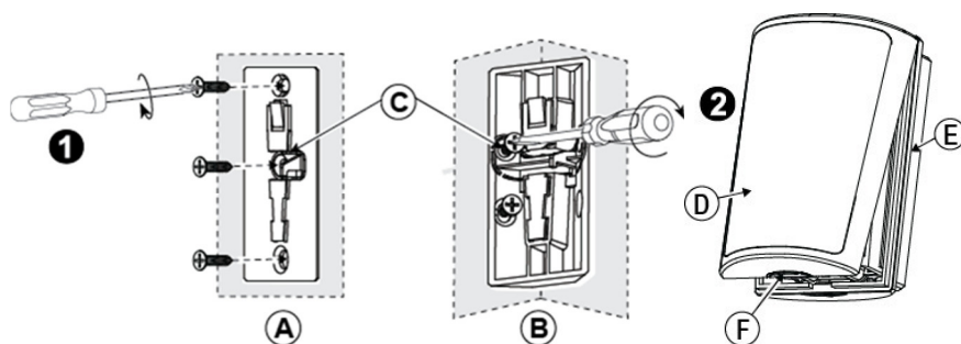
Figure 3 – Bracket Mounting
