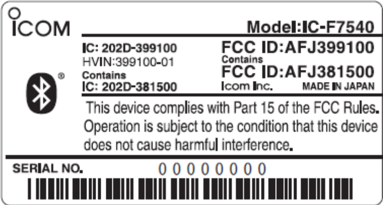
IC-F7540 Serial Plate
