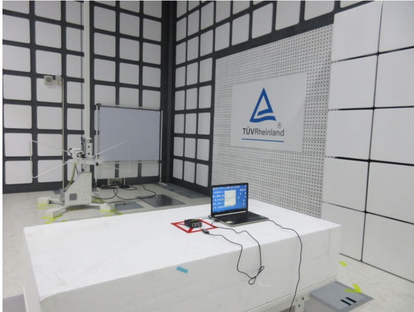
Photograph 3: Set-up for Spurious Emissions (Back View 1)
