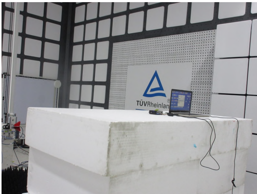
Photograph 4: Set-up for Spurious Emissions (Back View 2)
