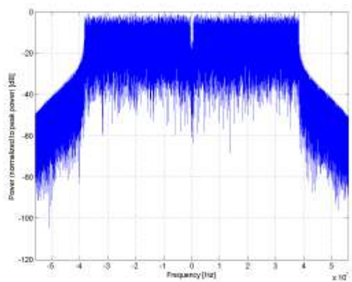
Frequency Domain
