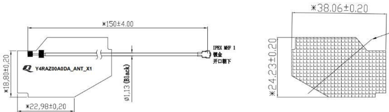
Antenna Dimensions
