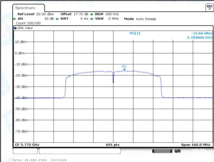
11AC80MIMO-Ant1-5775-PASS
