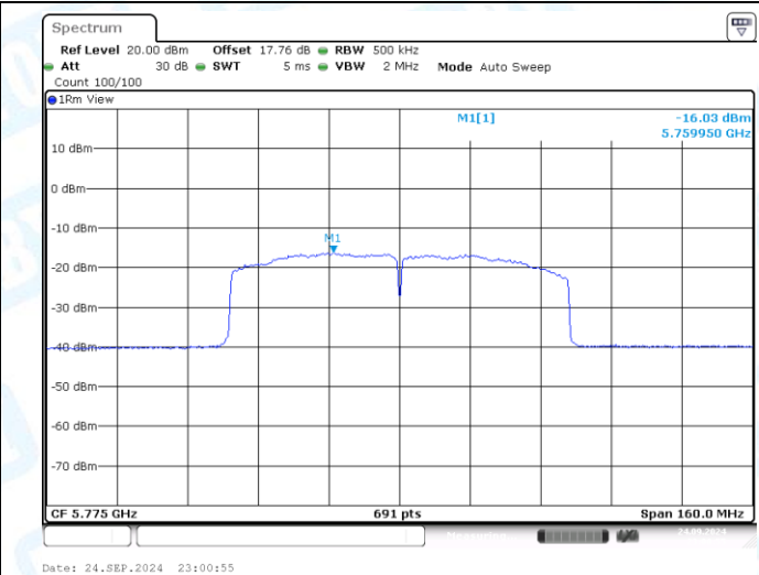
11AC80MIMO-Ant2-5775-PASS
