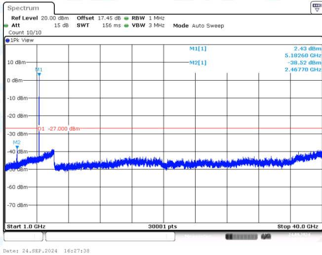
11A-CDD-Ant1-5180-1000~40000-PASS
