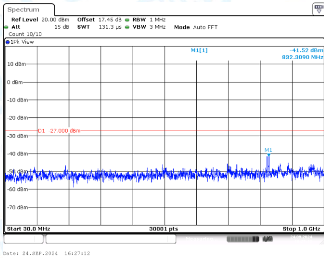
11A-CDD-Ant1-5180-30~1000-PASS
