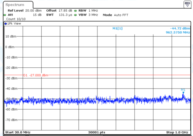
11AC20MIMO-Ant2-5825-30~1000-PASS
