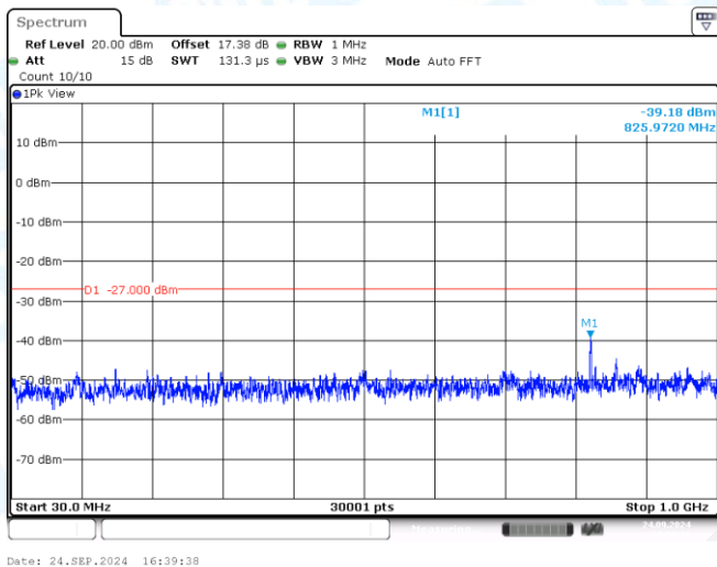
11A-CDD-Ant1-5200-30~1000-PASS
