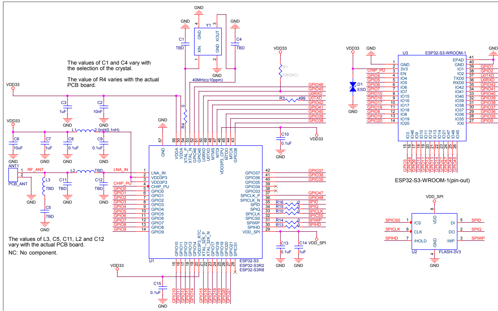
Figure 5: ESP32-S3-WROOM-1 Schematics
