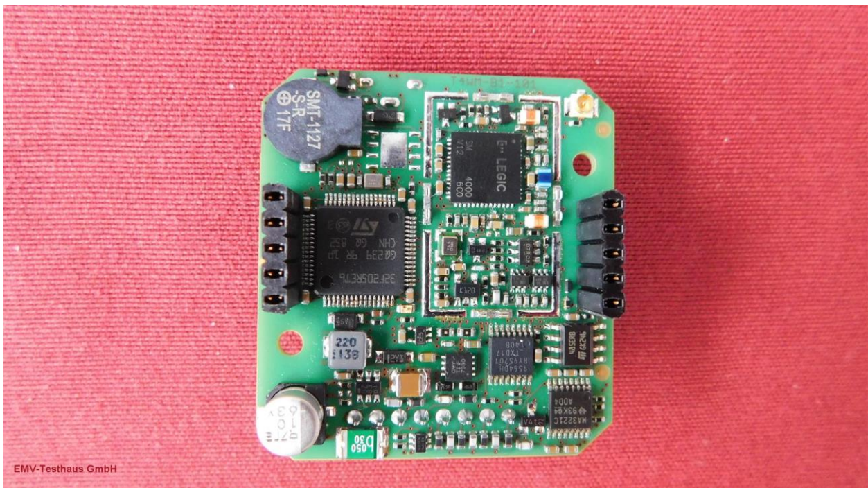
Picture 10: EUT – interface board - top view – without shielding
