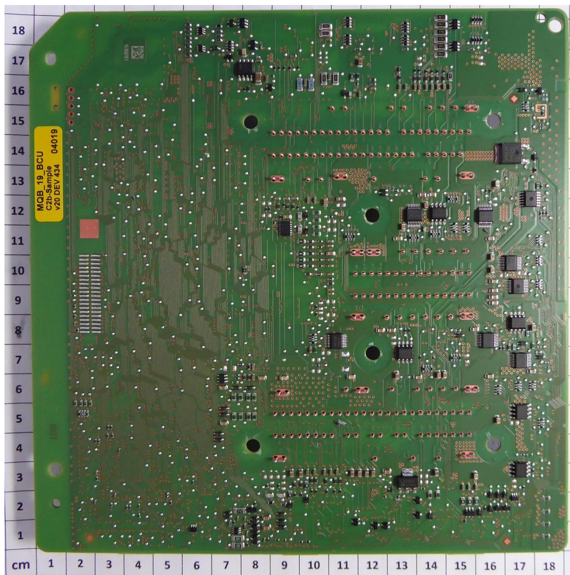
PCB front
