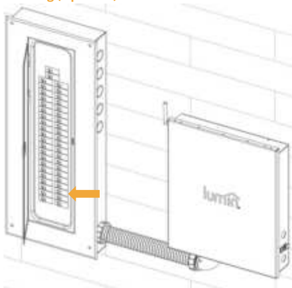
Completed Exterior Wall Mount Installation
