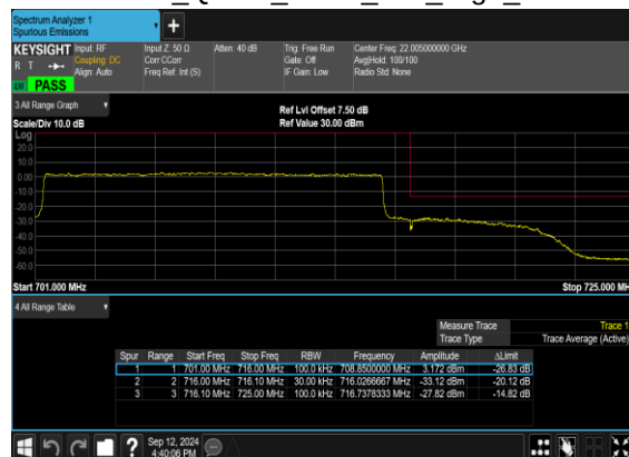
N12(15M)_DFT-s- OFDM QPSK Outer Full High CH
