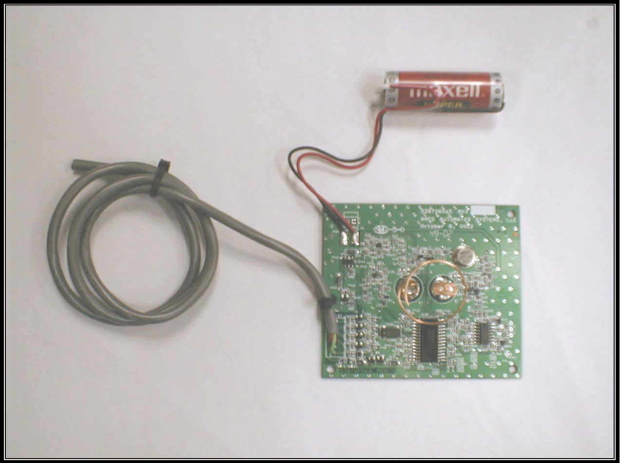
PHOTOGRAPH 5: FRONT VIEW OF TRANSPONDER
