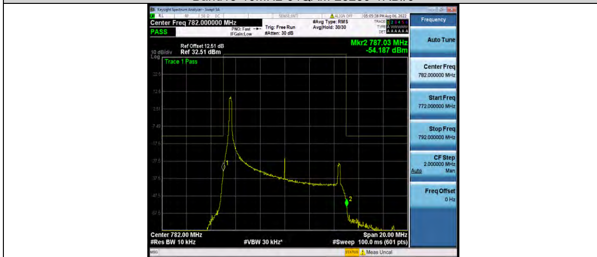
Band13-10MHz-64QAM-23230-1RB#49
