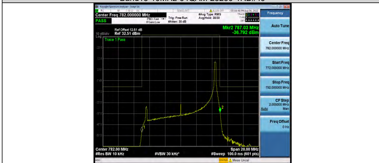
Band13-10MHz-64QAM-23230-50RB#0
