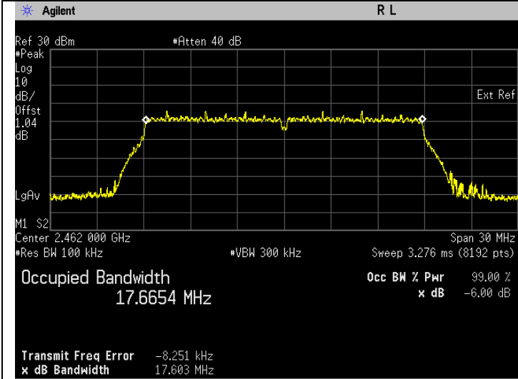
6dB Bandwidth. 802.11n Frequency 2462 MHz
