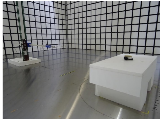
30 - 1000 MHz
