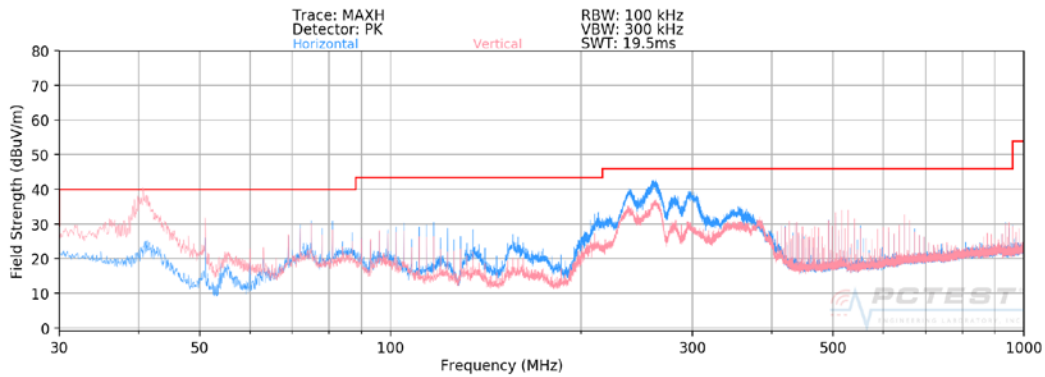
Plot 7-1. Radiated Spurious Plot below 1GHz
