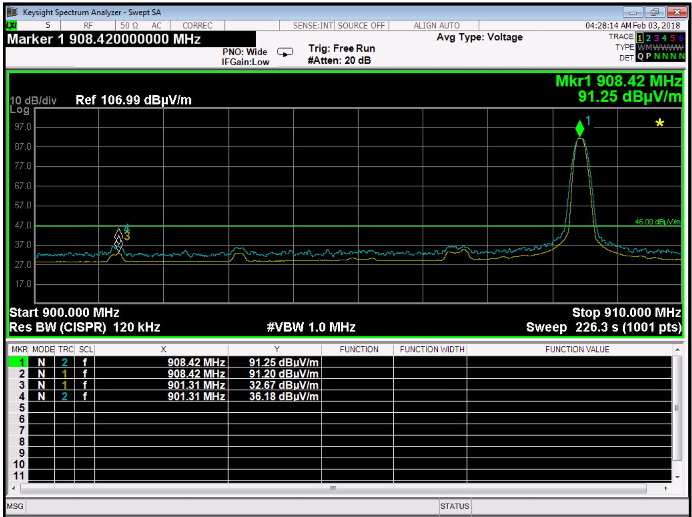
Band Edge - 908.42 MHz - Vertical - Y-Axis - Worst Case
