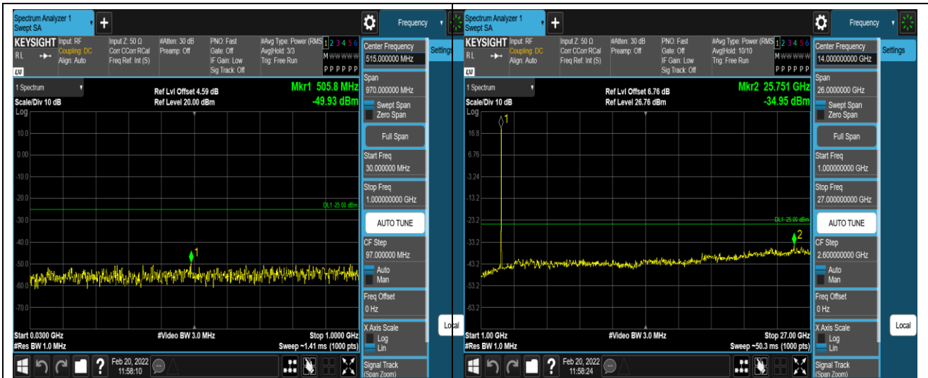
Band38-5MHz-16QAM-38225-1RB#0-Range1:30~1000MHz
