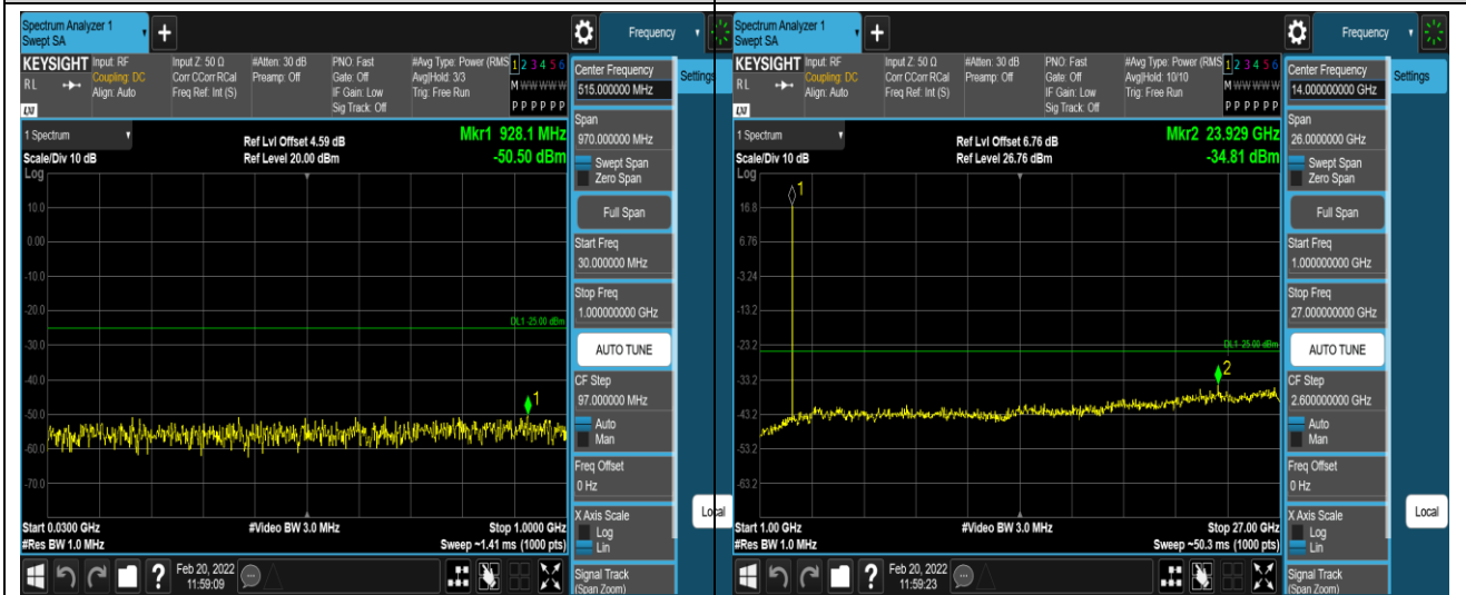
Band38-20MHz-QPSK-37850-1RB#0-Range1:30~1000MHz
