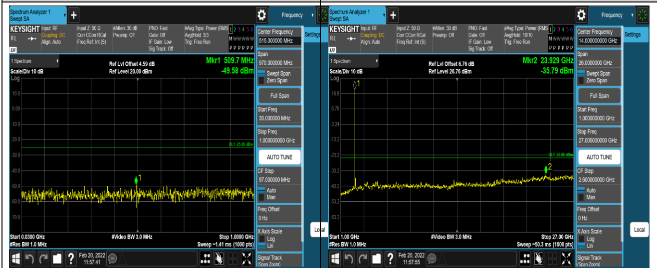
Band38-5MHz-QPSK-38000-1RB#0-Range1:30~1 000MHz
