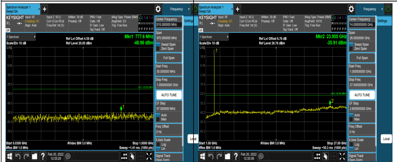
Band38-20MHz-QPSK-37850-1RB#0-Range1:30~1000MHz
