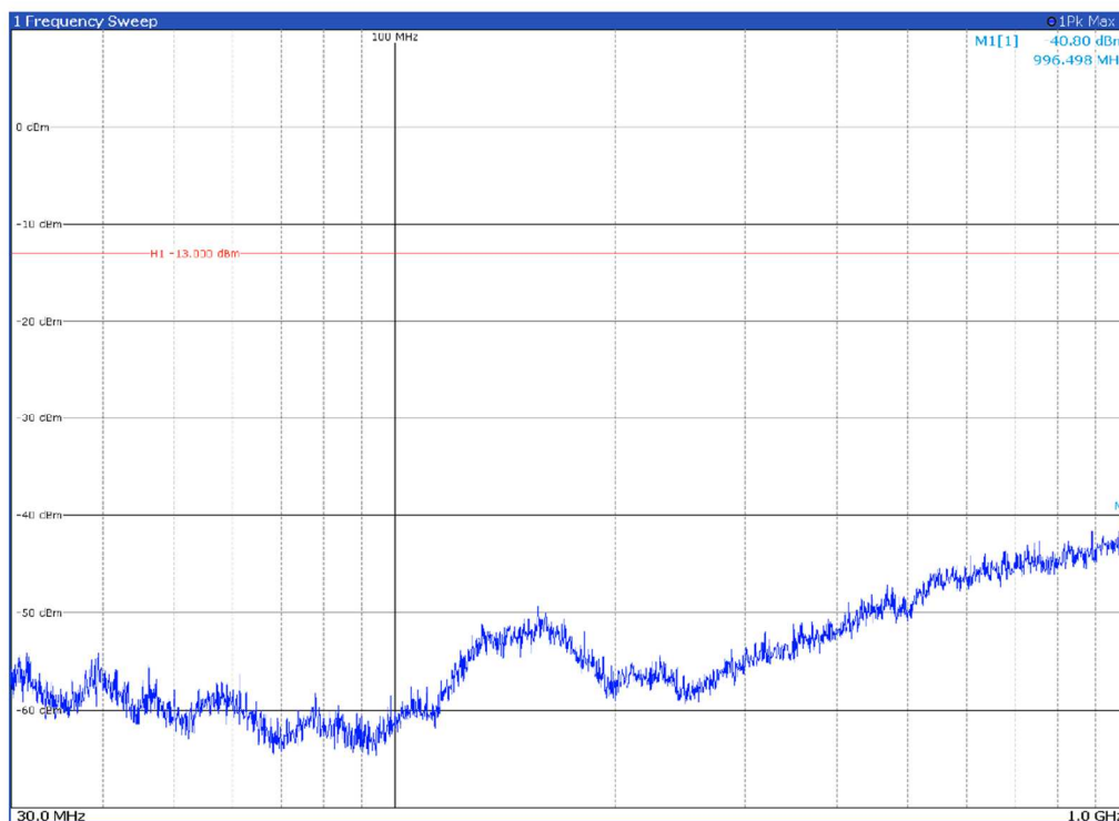
Channel: TOP, Modulation: 64QAM, BW=30MHz, Range: 30MHz - 1GHz, Polarization: Vertical
