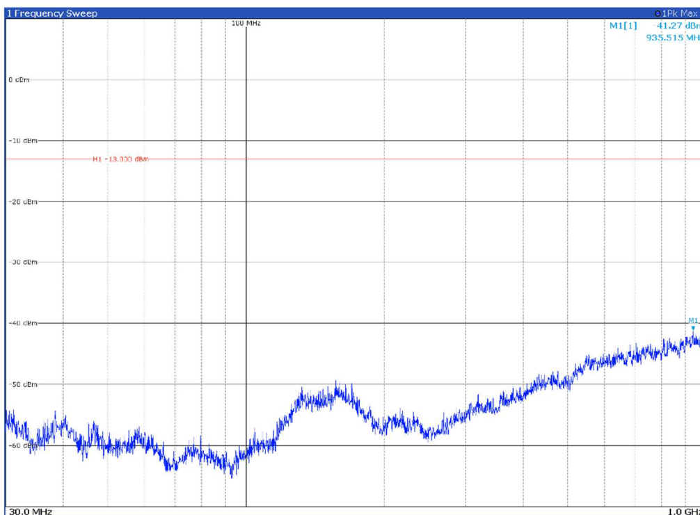
Channel: MIDDLE, Modulation: 64QAM, BW=40MHz, Range: 30MHz - 1GHz, Polarization: Vertical
