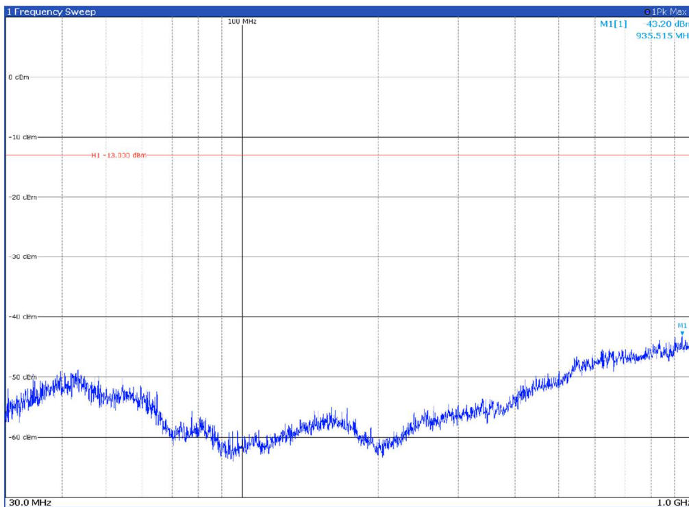
Channel: MIDDLE, Modulation: 64QAM, BW=40MHz, Range: 30MHz - 1GHz, Polarization: Horizontal
