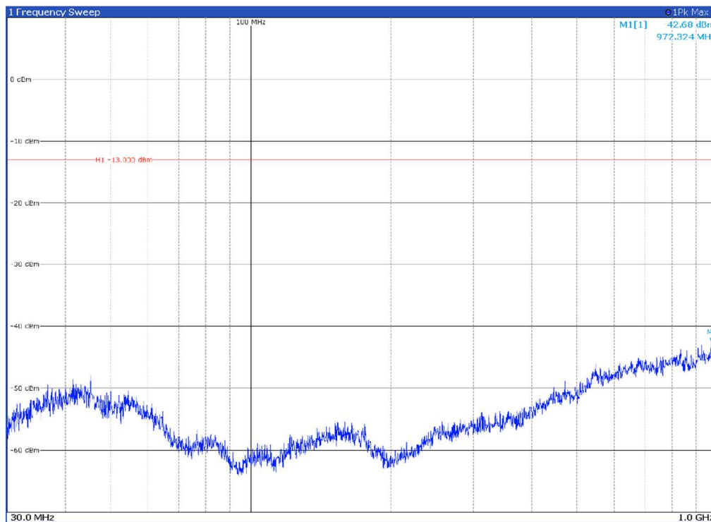
Channel: TOP, Modulation: 64QAM, BW=30MHz, Range: 30MHz - 1GHz, Polarization: Horizontal
