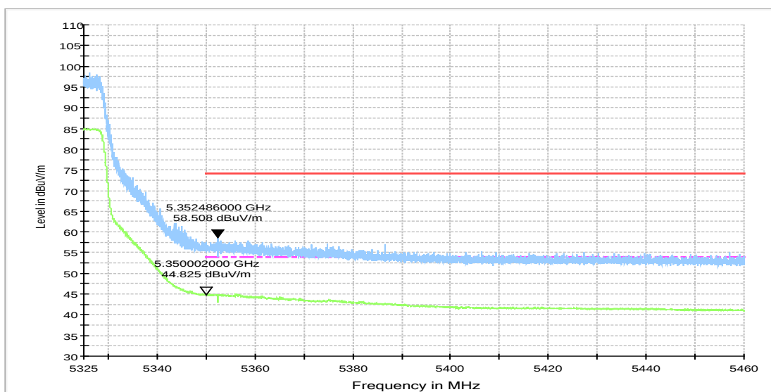
Fig.54 Band Edges (802.11ax-HT80, 5290MHz)
