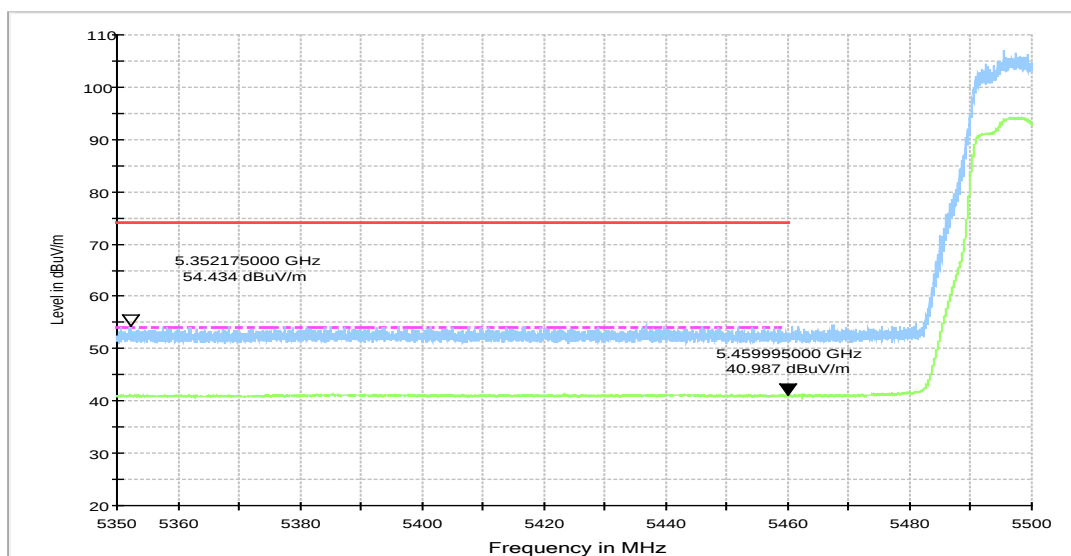
Fig.15 Band Edges (802.11ax-HT20, 5500MHz)
