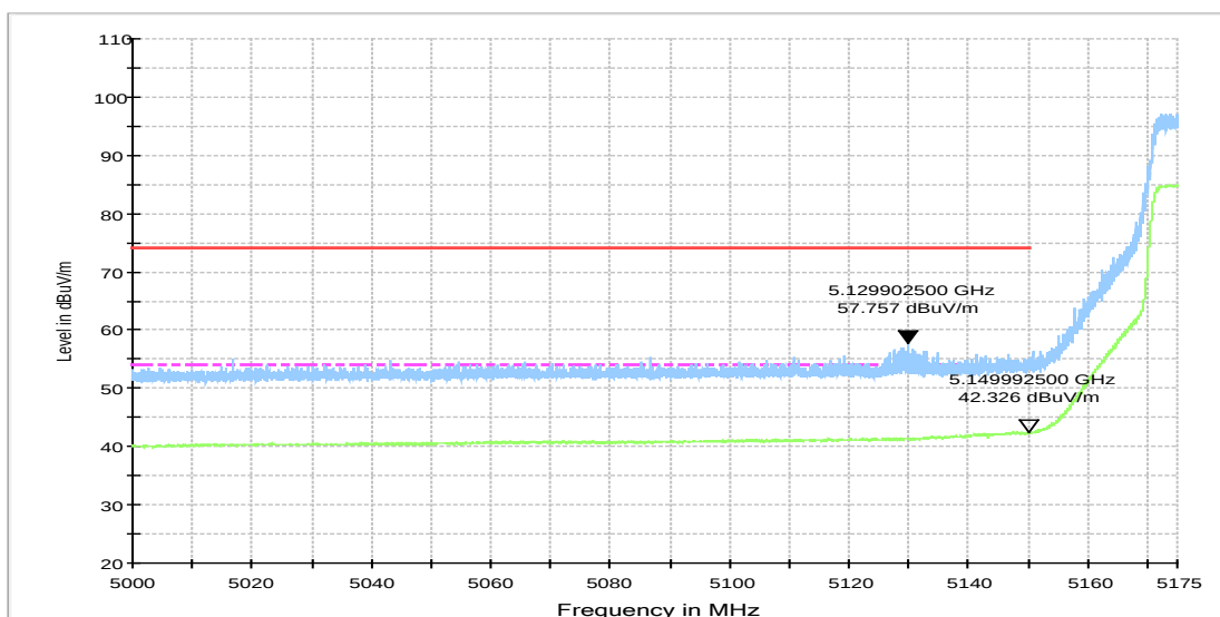
Fig.53 Band Edges (802.11ax-HT80, 5210MHz)
