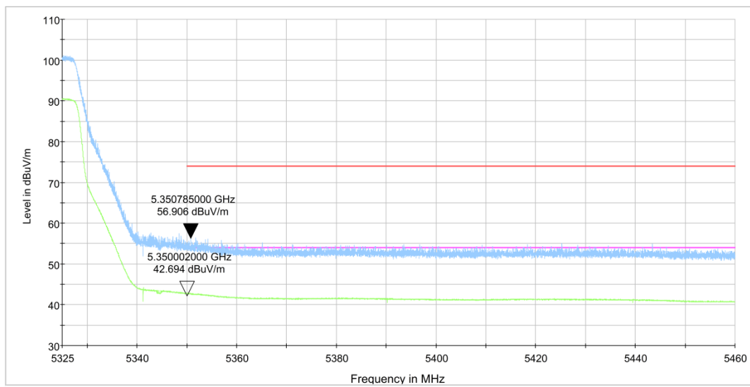
Fig.10 Band Edges (802.11n-HT40, 5310MHz)
