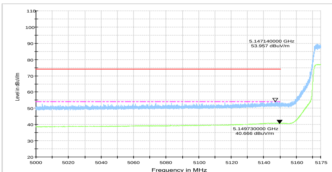
Fig.21 Band Edges (802.11ax-HT80, 5210MHz)
