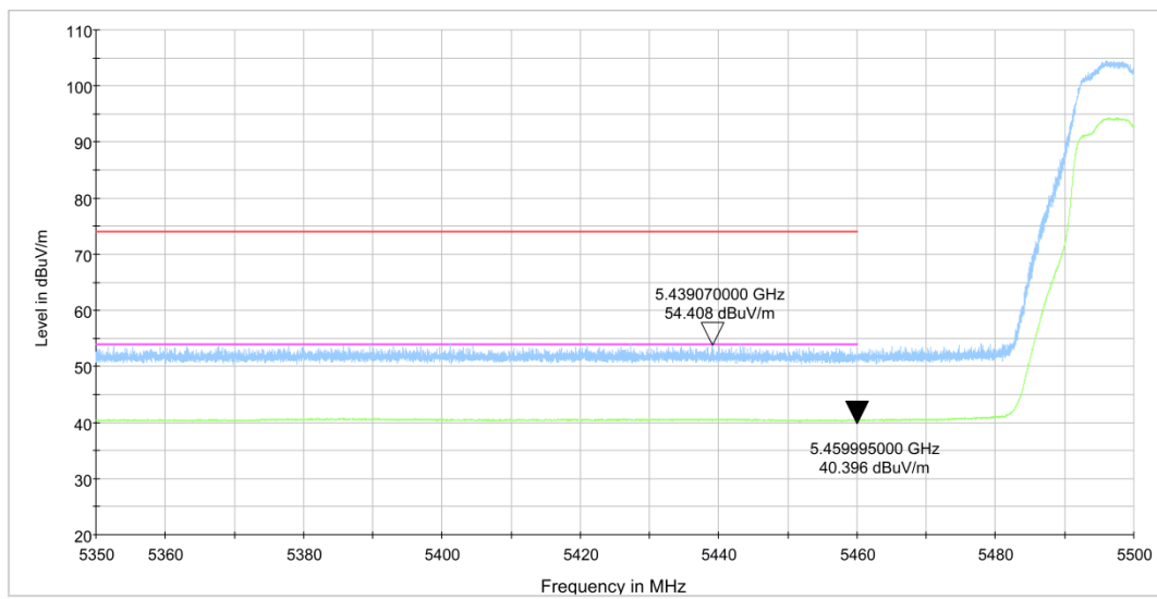
Fig.3 Band Edges (802.11a, 5500MHz)
