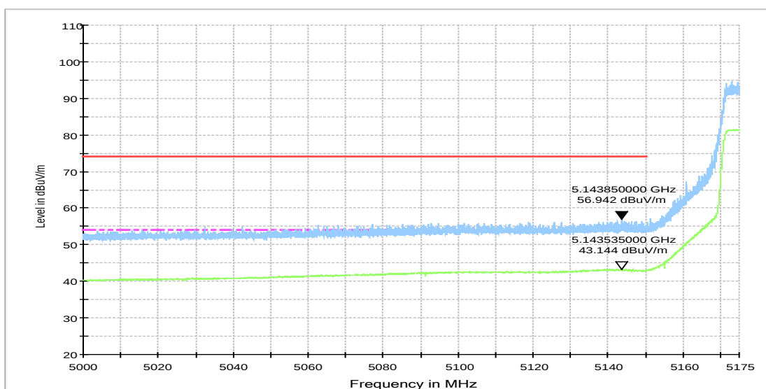
Fig.56 Band Edges (802.11ax-HT160, 5250MHz)
