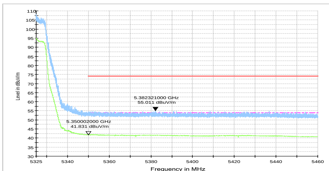
Fig.14 Band Edges (802.11ax-HT20, 5320MHz)
