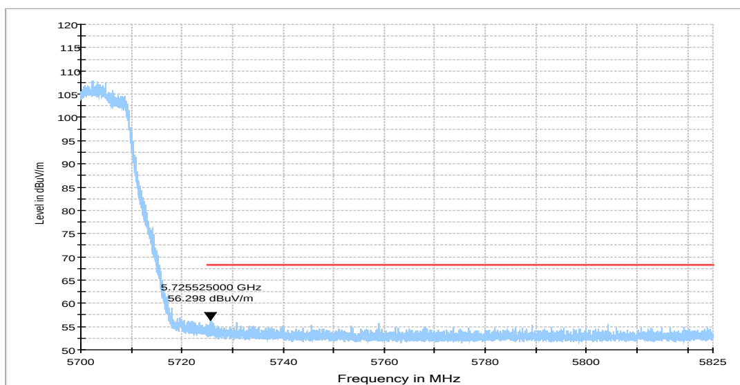
Fig.16 Band Edges (802.11ax-HT20, 5700MHz)
