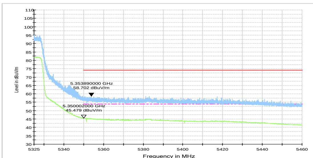
Fig.57 Band Edges (802.11ax-HT160, 5250MHz)
