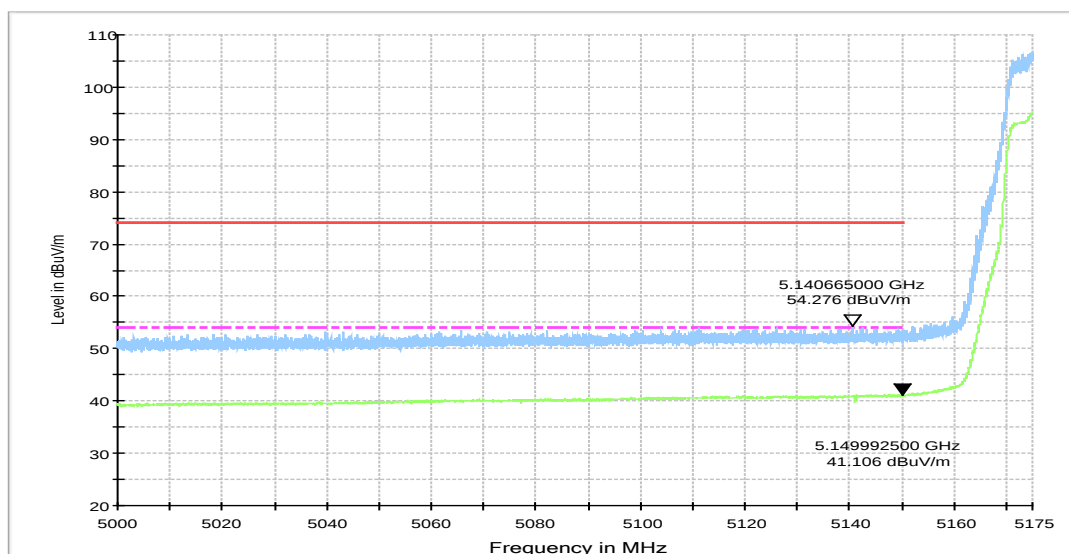
Fig.13 Band Edges (802.11ax-HT20, 5180MHz)
