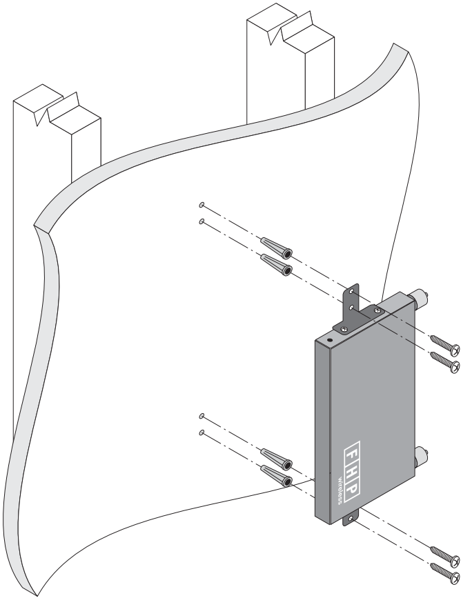
Figure 5 Flat Mounting Option
