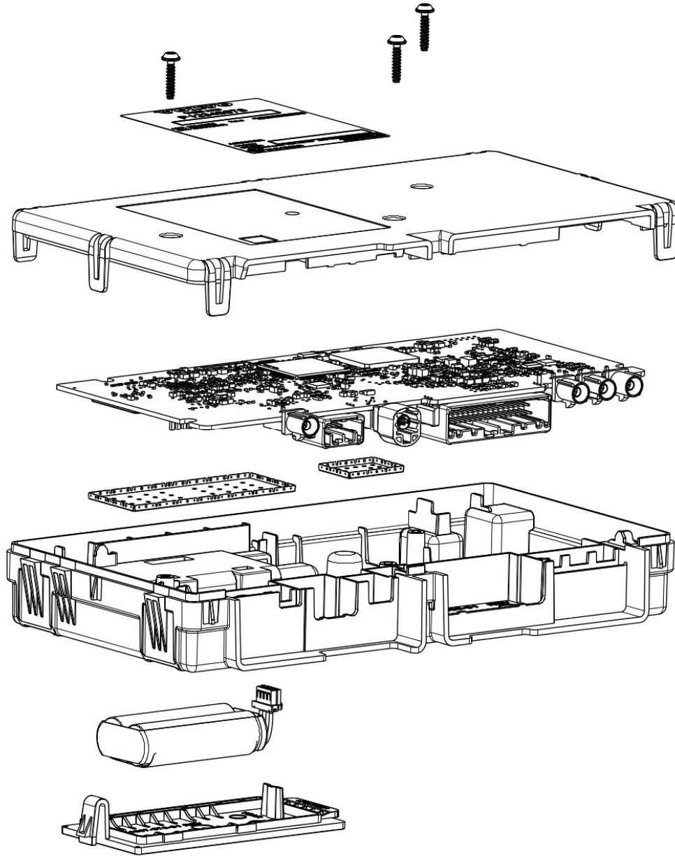
Figure 1 – Mechanical design
