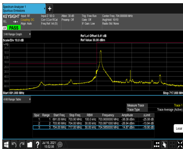
Band17-10MHz-16QAM-23780-50RB#0
