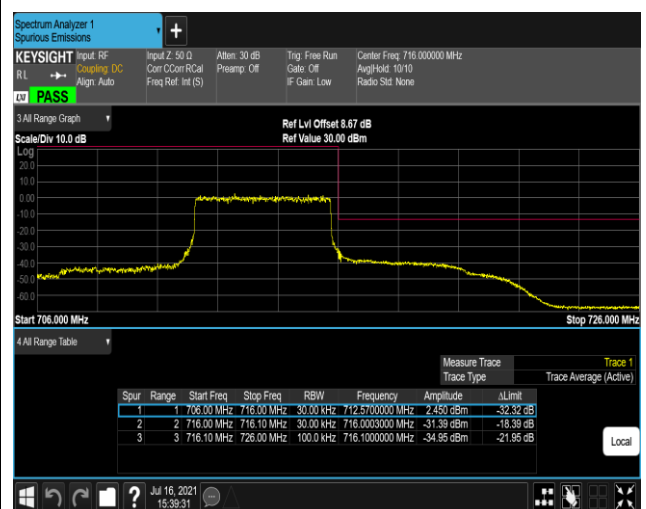
Band17-5MHz-QPSK-23825-25RB#0
