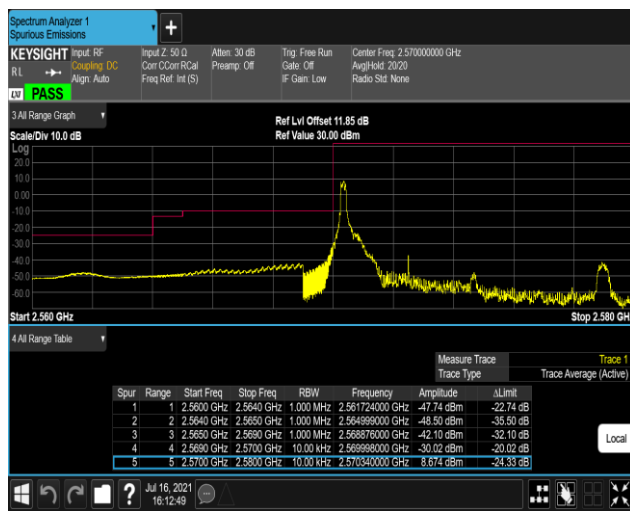
Band38-5MHz-16QAM-37775-25RB#0
