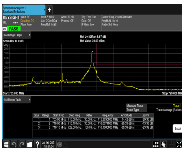
Band17-10MHz-16QAM-23800-1RB#49
