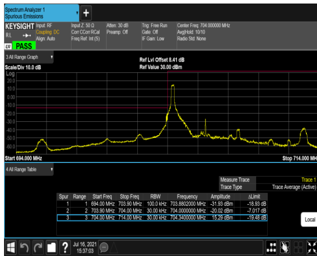
Band17-5MHz-QPSK-23755-25RB#0
