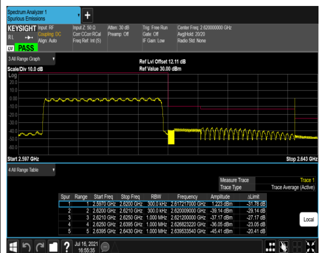
Band38-20MHz-QPSK-38150-100RB#0
