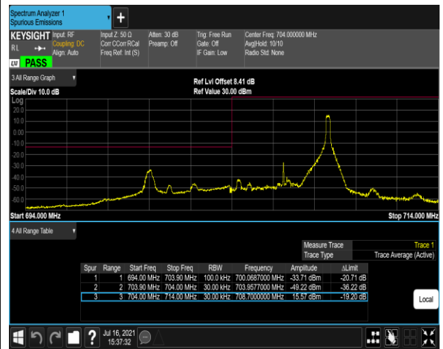
Band17-5MHz-QPSK-23825-1RB#0
