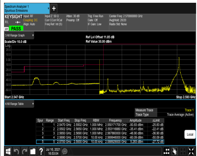
Band38-20MHz-16QAM-38150-1RB#0
