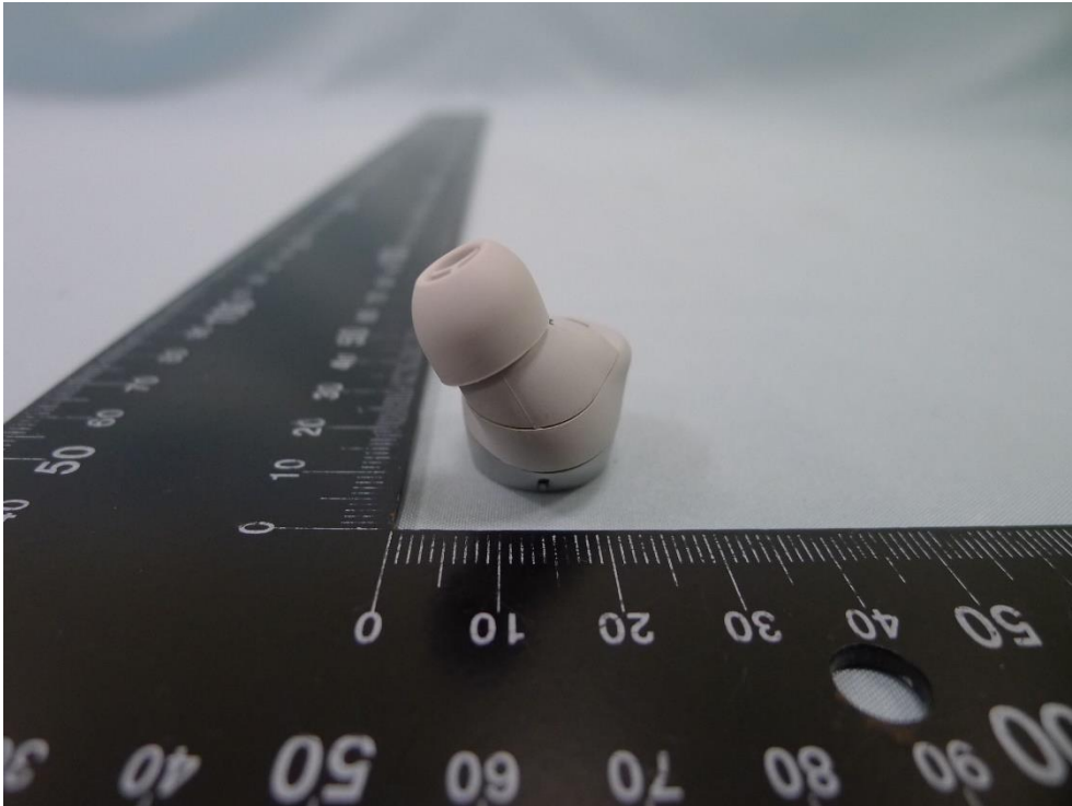
(15) EUT Photo (Right Ear_ Silver)
