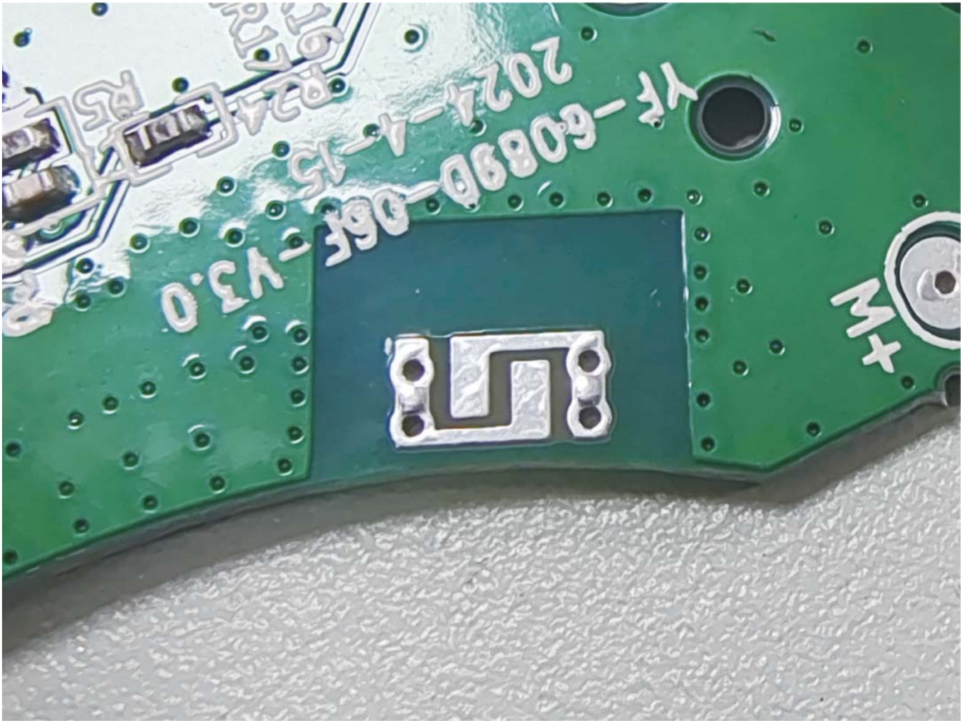
Antenna physical and physical dimensions
