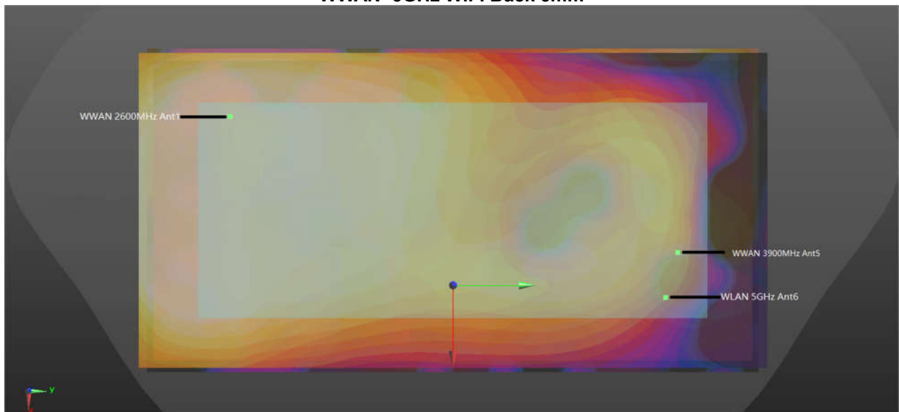
WWAN+5GHz WIFI Front 5mm
