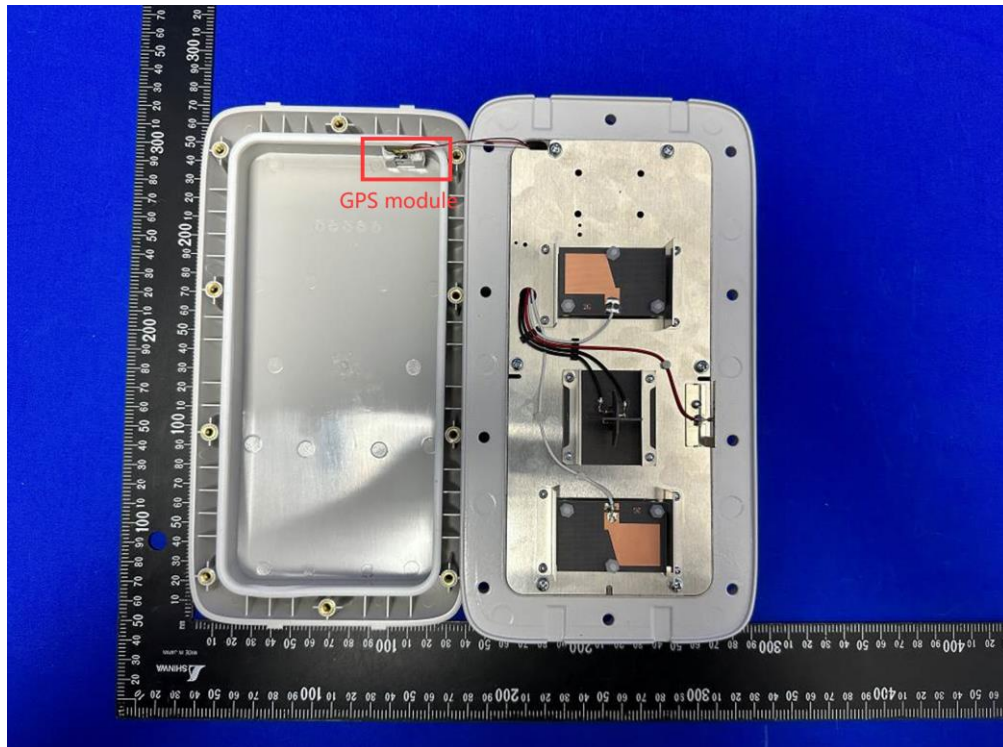
(1) EUT Photo (WF-660AG, with GPS module)
