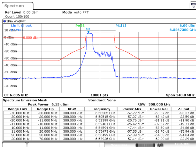
SISO-B, 802.11ax/be20-MCS0, Ch117-4m-37
