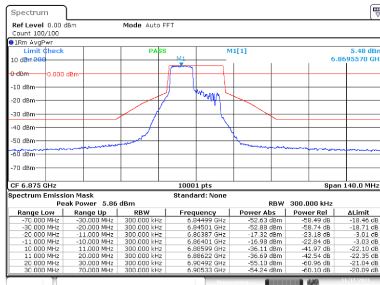
SISO-B, 802.11ax/be20-MCS0, Ch185-8m-53
