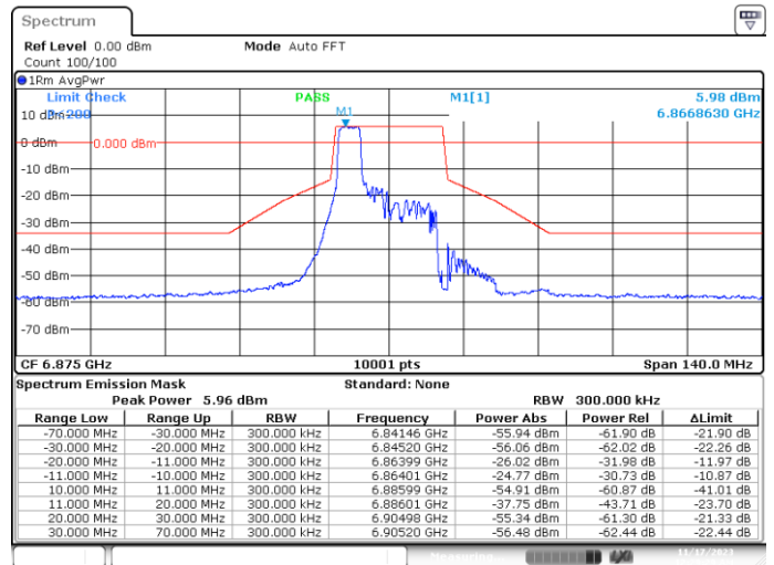
SISO-B, 802.11ax/be20-MCS0, Ch185-4m-37
