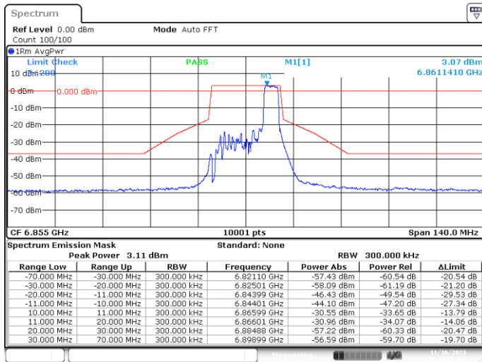
MIMO-A, 802.11ax/be20-MCS0, Ch181-4m-37
