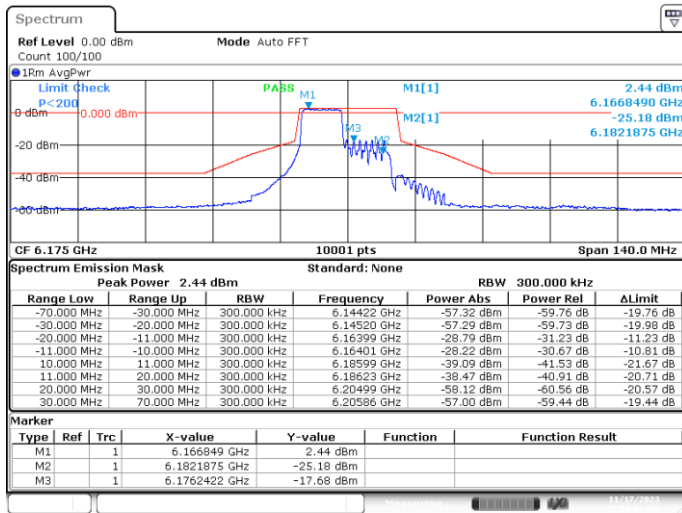
MIMO-B, 802.11ax/be20-MCS0, Ch45-8m-53
