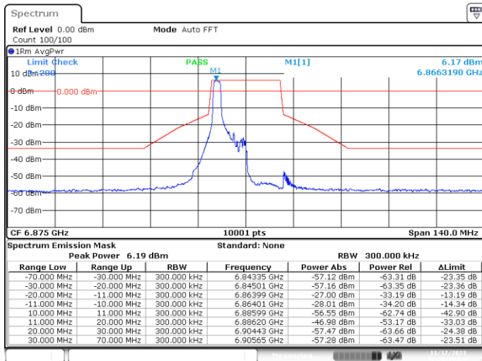
SISO-B, 802.11ax/be20-MCS0, Ch185-2m-0
