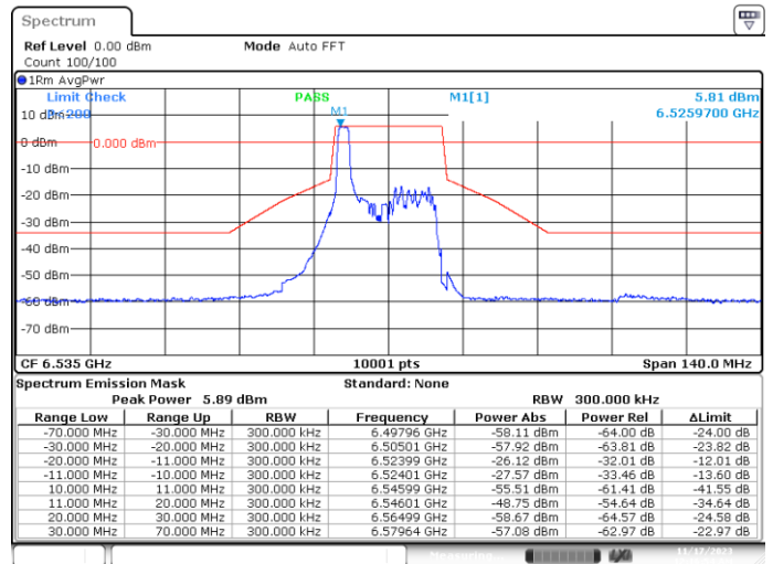
SISO-B, 802.11ax/be20-MCS0, Ch117-2m-0
