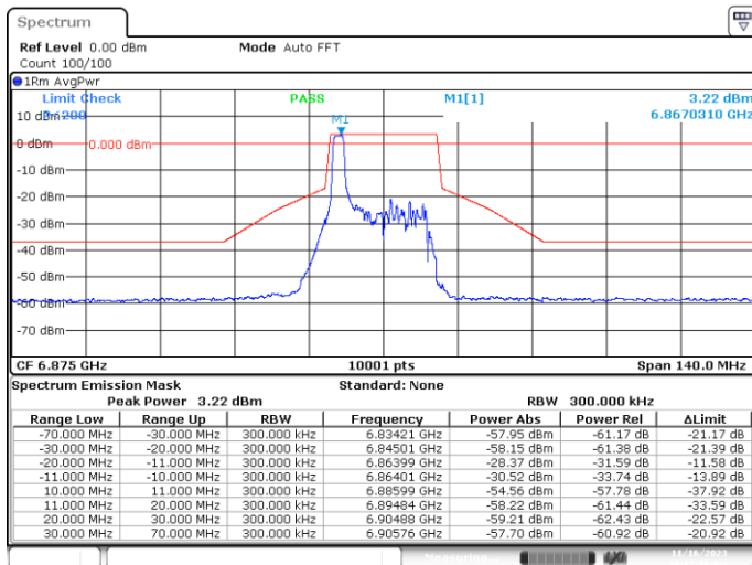
MIMO-A, 802.11ax/be20-MCS0, Ch185-2m-0
