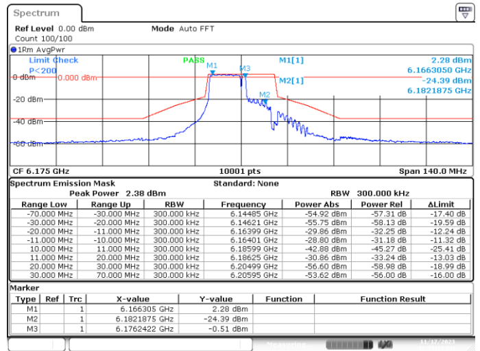
MIMO-B, 802.11ax/be20-MCS0, Ch45-10m-82
