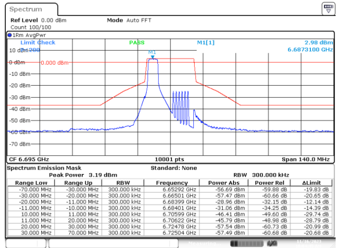
MIMO-A, 802.11ax/be20-MCS0, Ch149-4m-37
