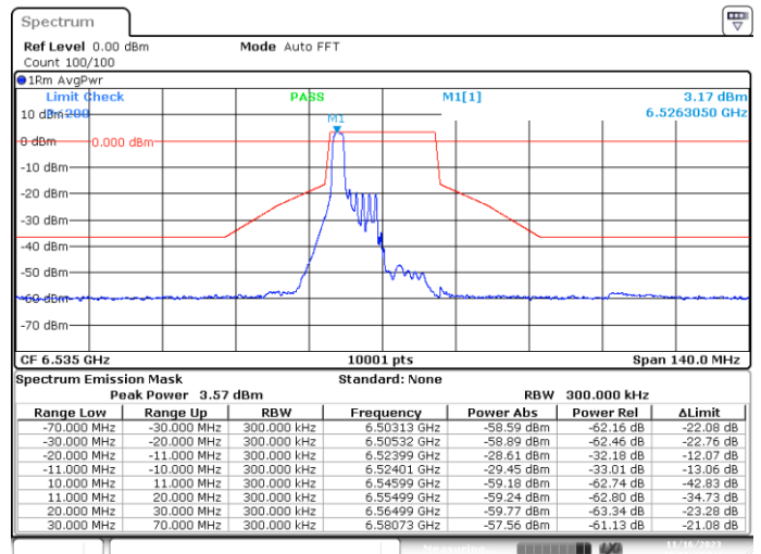
MIMO-A, 802.11ax/be20-MCS0, Ch117-2m-0
