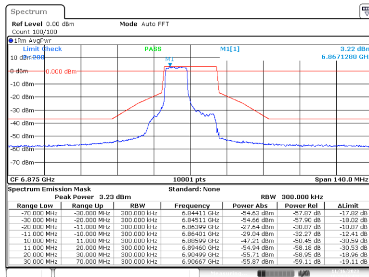
MIMO-A, 802.11ax/be20-MCS0, Ch185-8m-53
