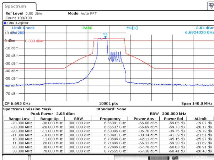
MIMO-A, 802.11ax/be20-MCS0, Ch149-6m-70
