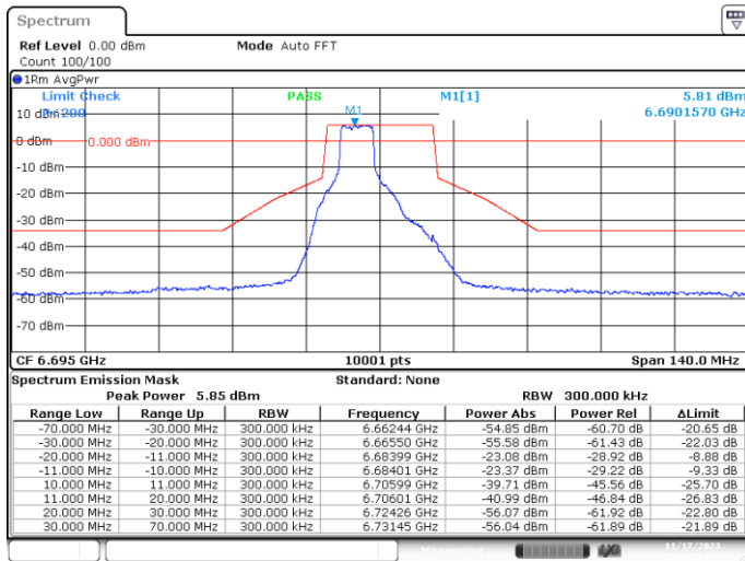
SISO-B, 802.11ax/be20-MCS0, Ch149-6m-70
