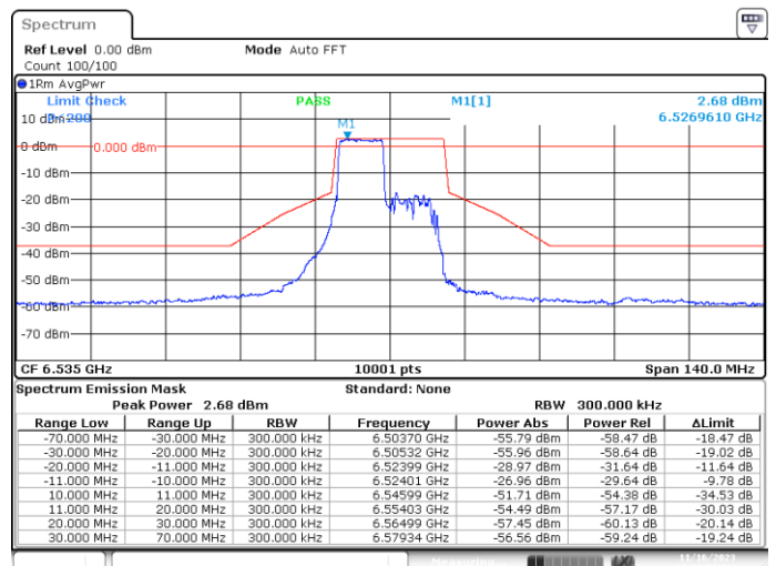
MIMO-A, 802.11ax/be20-MCS0, Ch117-8m-53
