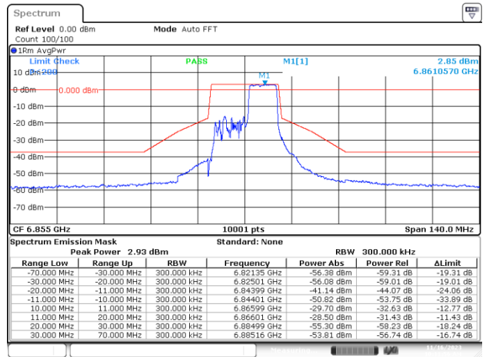
MIMO-A, 802.11ax/be20-MCS0, Ch181-8m-53
