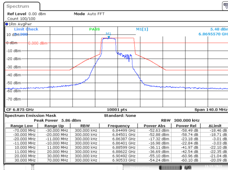
SISO-A, 802.11ax/be20-MCS0, Ch185-8m-53
