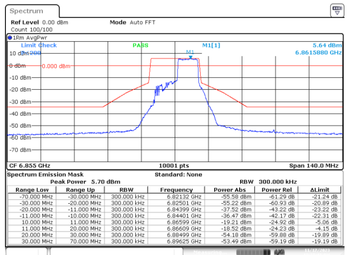
SISO-B, 802.11ax/be20-MCS0, Ch181-8m-53
