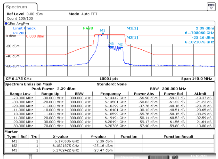
MIMO-B, 802.11ax/be20-MCS0, Ch45-6m-70
