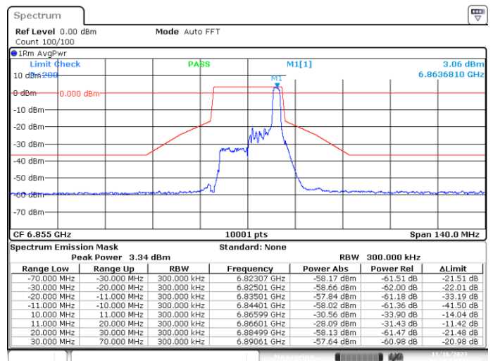
MIMO-A, 802.11ax/be20-MCS0, Ch181-2m-0
