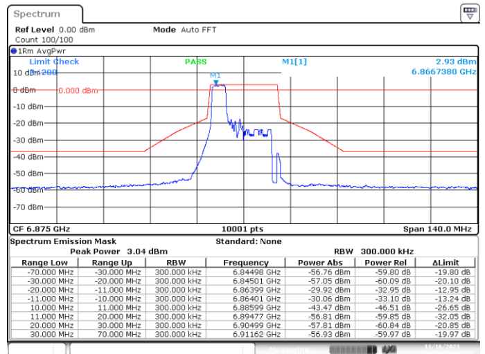
MIMO-A, 802.11ax/be20-MCS0, Ch185-4m-37
