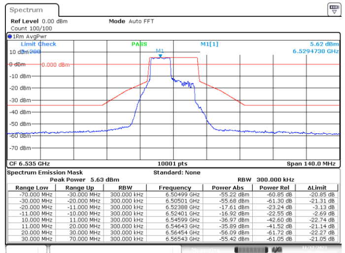
SISO-B, 802.11ax/be20-MCS0, Ch117-8m-53
