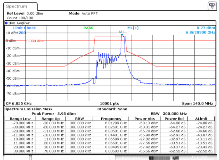
SISO-B, 802.11ax/be20-MCS0, Ch181-2m-0
