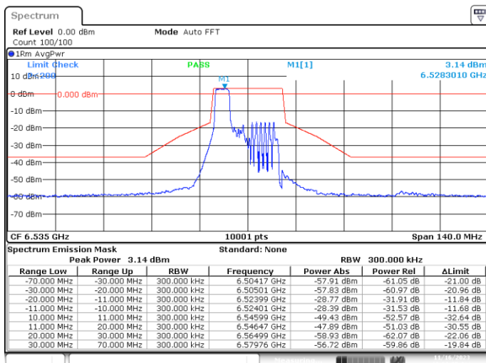
MIMO-A, 802.11ax/be20-MCS0, Ch117-4m-37
