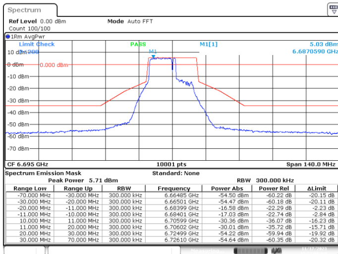
SISO-B, 802.11ax/be20-MCS0, Ch149-10m-82
