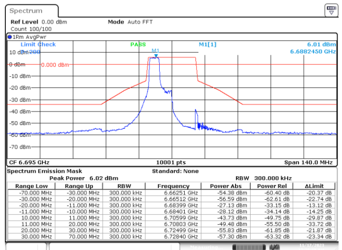
SISO-B, 802.11ax/be20-MCS0, Ch149-4m-37
