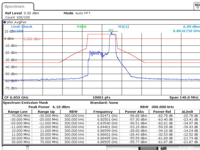
SISO-B, 802.11ax/be20-MCS0, Ch181-4m-37
