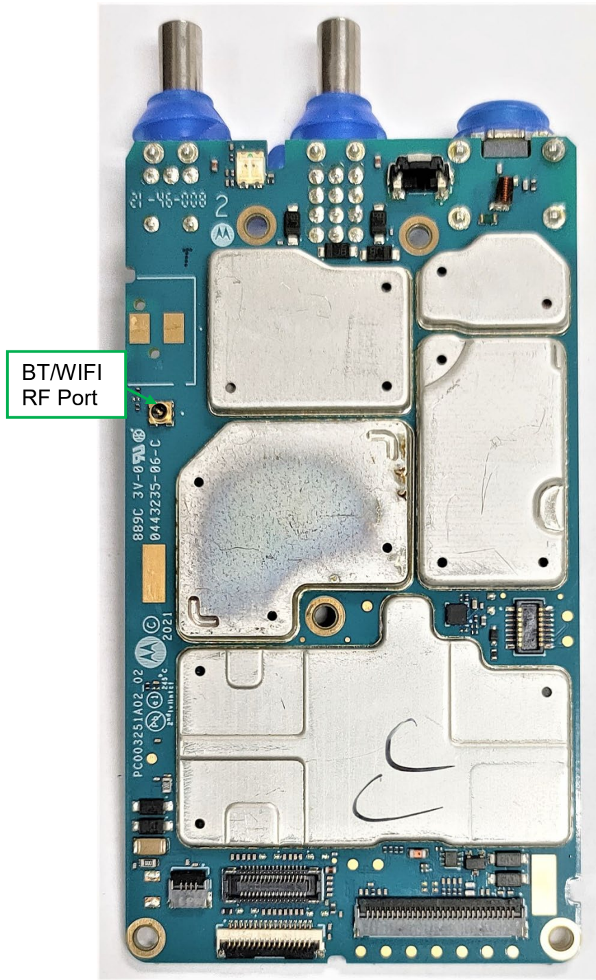
RF Board With Shields (Top) TIA4950
