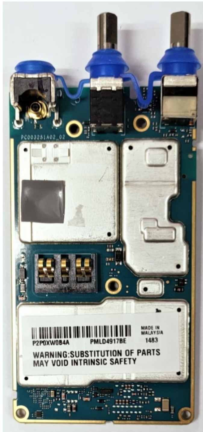
RF Board With Shields (Bottom) TIA4950
