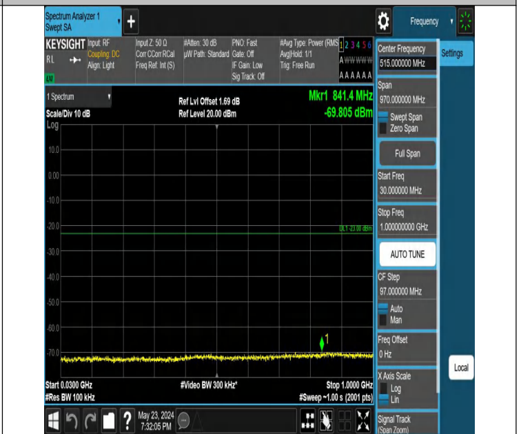
Band66_20MHz_QPSK_132322_1RB#99_30~1000_30~1000
