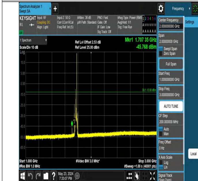
Band66_20MHz_QPSK_132572_1RB#99_1000~3000_1000~300
