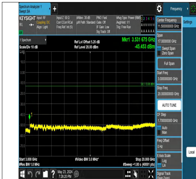
Band66_15MHz_QPSK_132597_1RB#0_3000~20000_3000~20000
