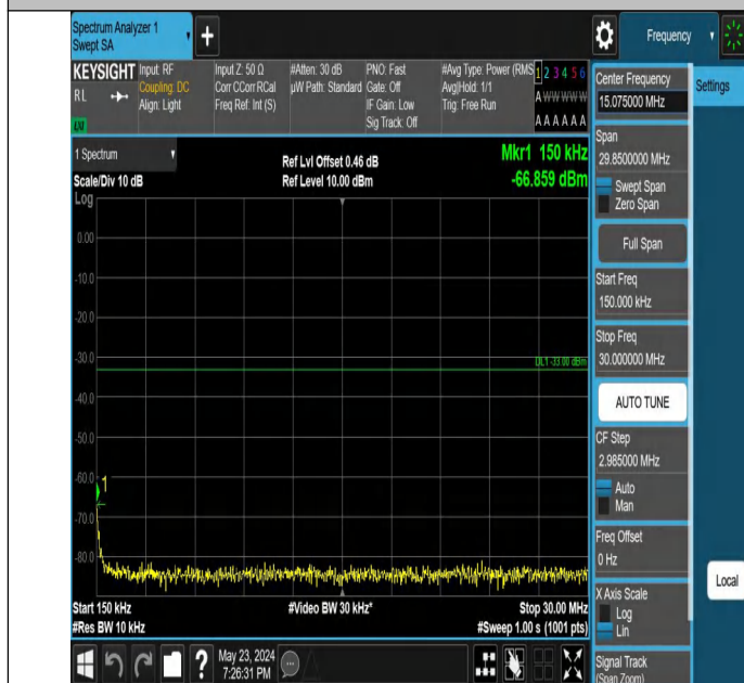
Band66_15MHz_QPSK_132597_1RB#74_0.15~30_0.15~30
