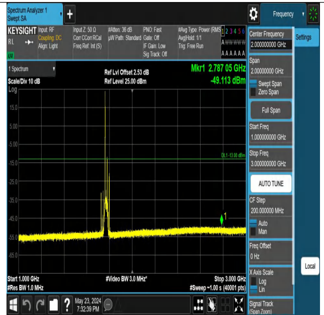
Band66_20MHz_QPSK_132572_1RB#0_1000~3000_1000~3000
