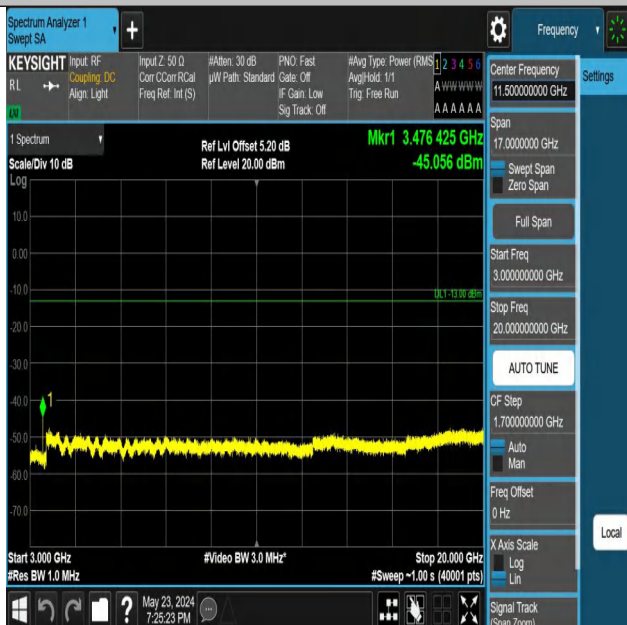
Band66_15MHz_QPSK_132322_1RB#0_3000~20000_3000~200
