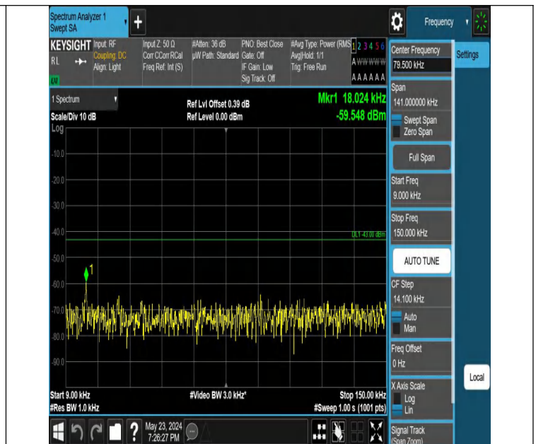
Band66_15MHz_QPSK_132597_1RB#74_0.009~0.15_0.009~0.15
