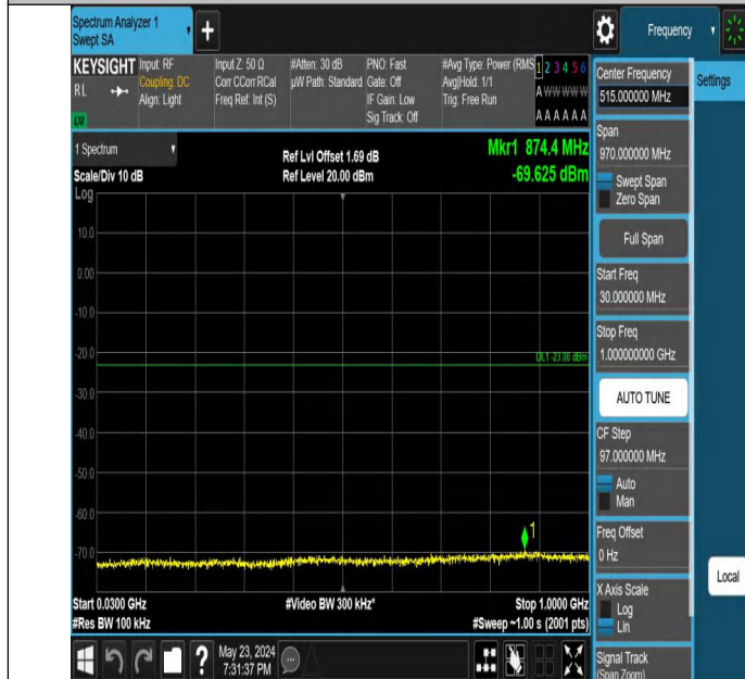
Band66_20MHz_QPSK_132322_1RB#0_30~1000_30~1000
