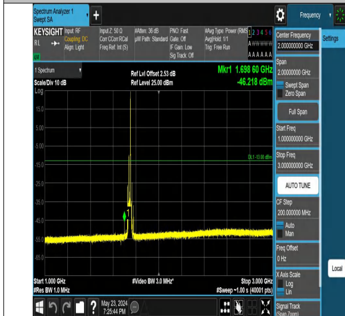
Band66_15MHz_QPSK_132322_1RB#74_1000~3000_1000~300
