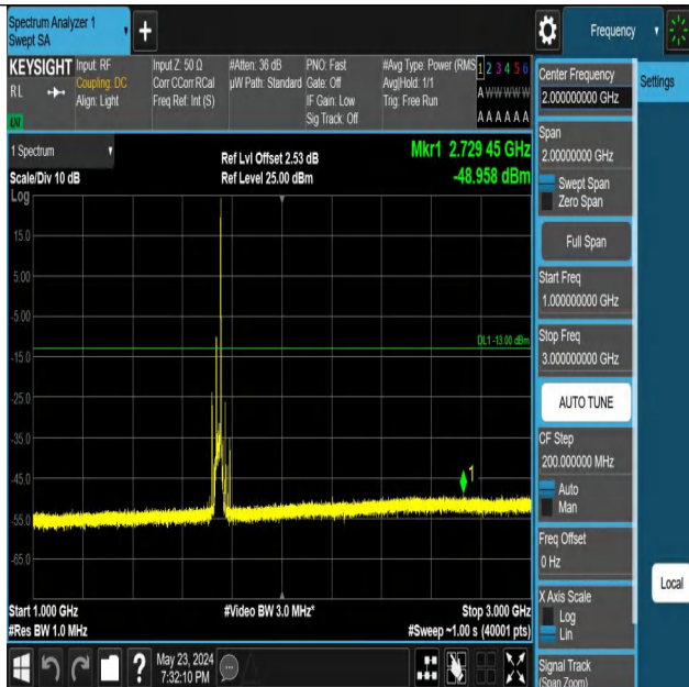
Band66_20MHz_QPSK_132322_1RB#99_1000~3000_1000~300
