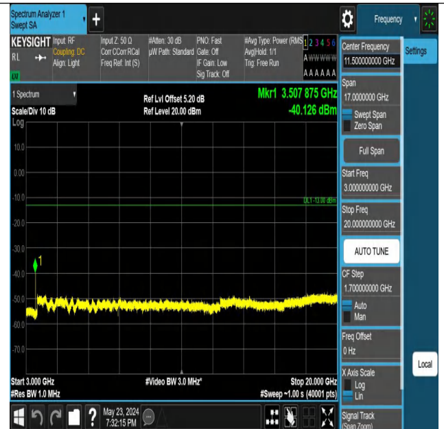
Band66_20MHz_QPSK_132322_1RB#99_3000~20000_3000~200
