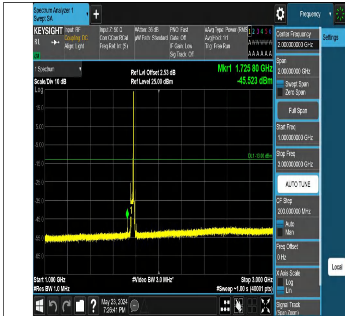
Band66_15MHz_QPSK_132597_1RB#74_1000~3000_1000~300
