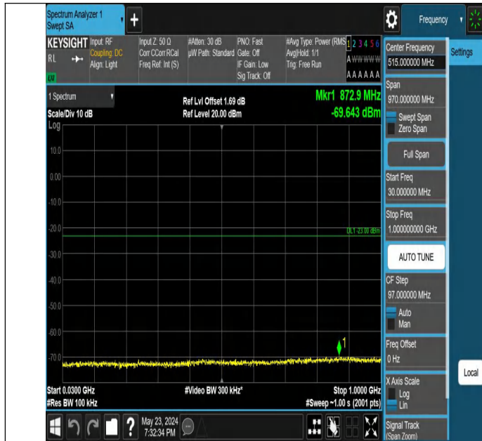
Band66_20MHz_QPSK_132572_1RB#0_30~1000_30~1000
