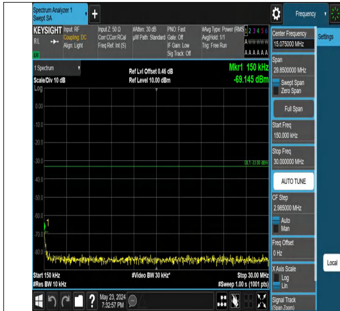
Band66_20MHz_QPSK_132572_1RB#99_0.15~30_0.15~30
