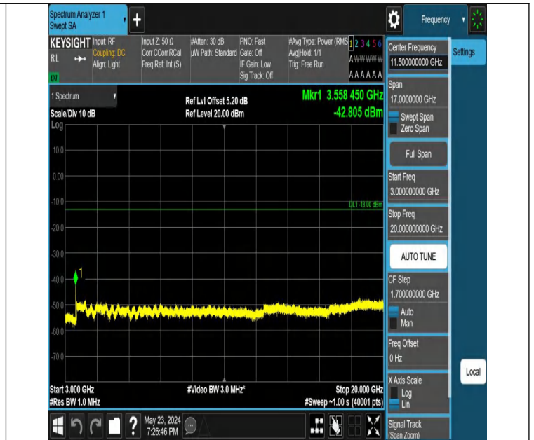
Band66_15MHz_QPSK_132597_1RB#74_3000~20000_3000~200
