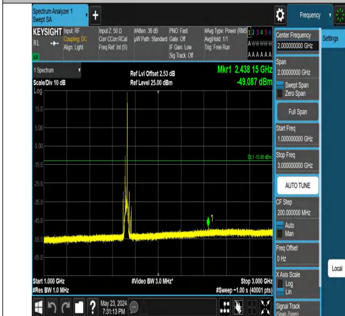
Band66_20MHz_QPSK_132072_1RB#99_1000~3000_1000~300
