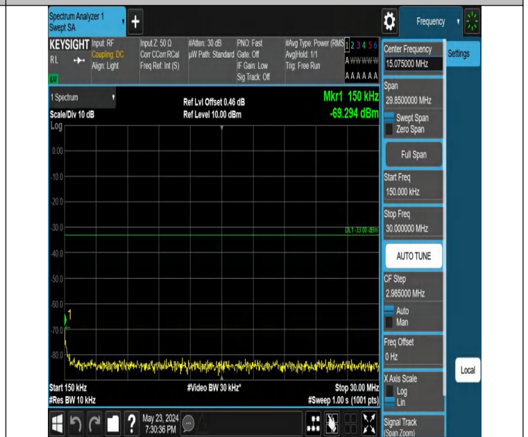
Band66_20MHz_QPSK_132072_1RB#0_0.15~30_0.15~30
