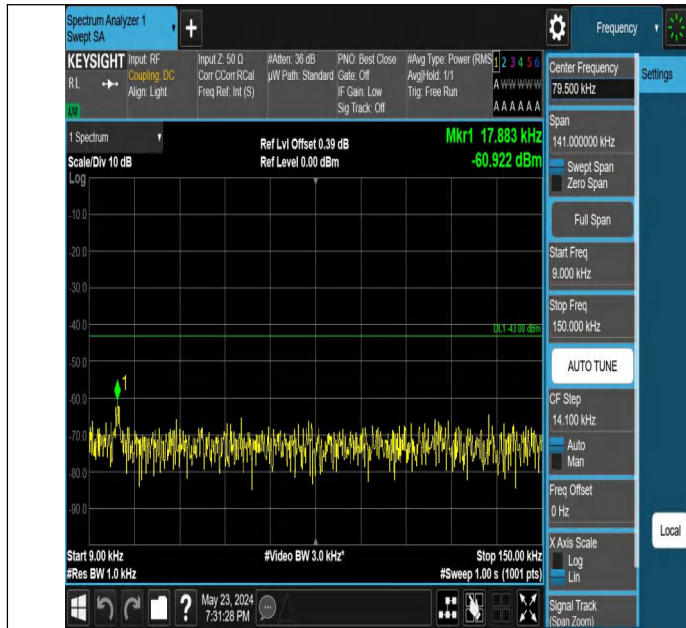
Band66_20MHz_QPSK_132322_1RB#0_0.009~0.15_0.009~0.15
