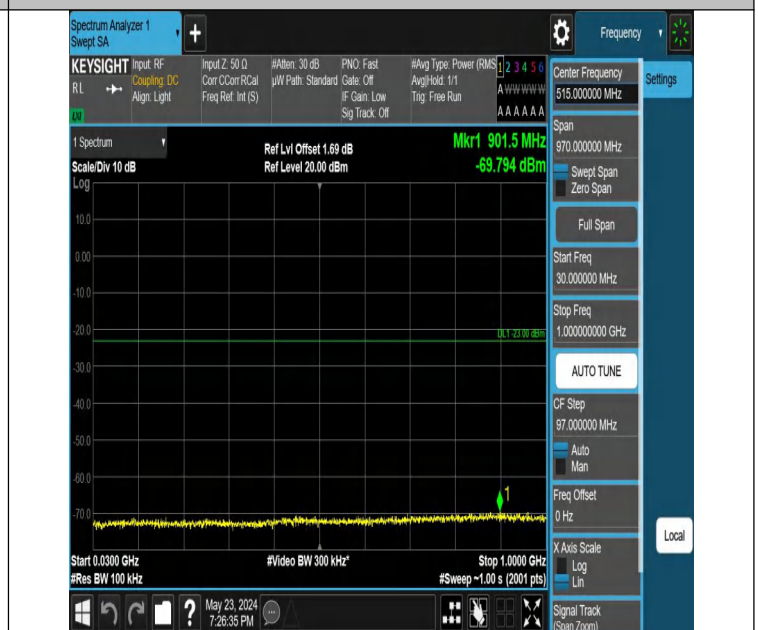
Band66_15MHz_QPSK_132597_1RB#74_30~1000_30~1000
