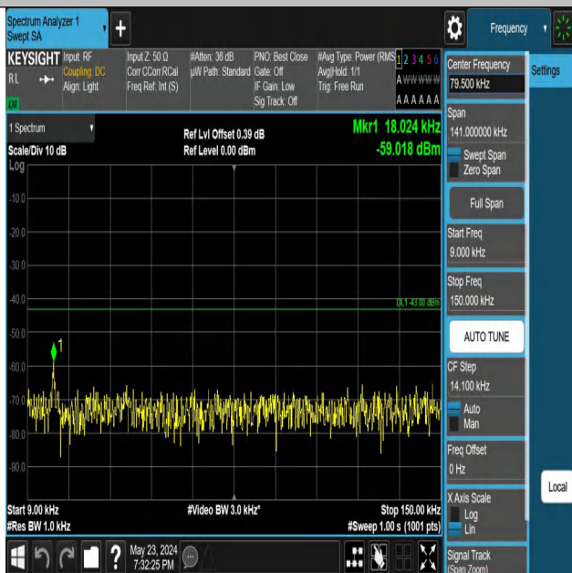
Band66 20MHz QPSK 132572 1RB#0 0.009~0.15 0.009~0.15
