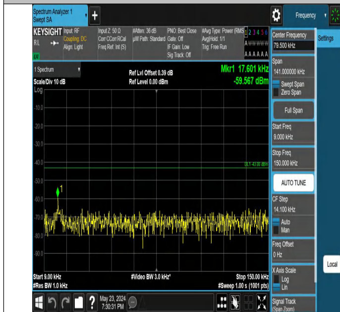
Band66_20MHz_QPSK_132072_1RB#0_0.009~0.15_0.009~0.15
