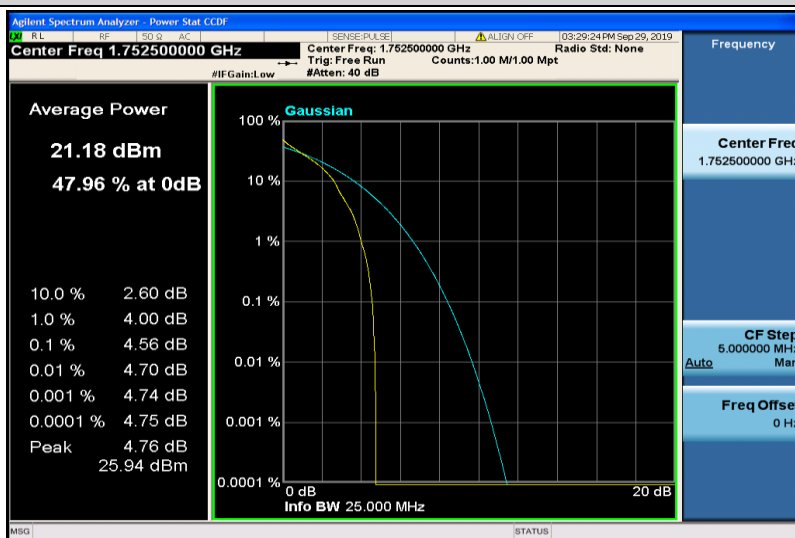
Band4-5MHz-QPSK-20375-1RB#0
