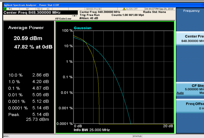
Band5-1.4MHz-16QAM-20643-1RB#0
