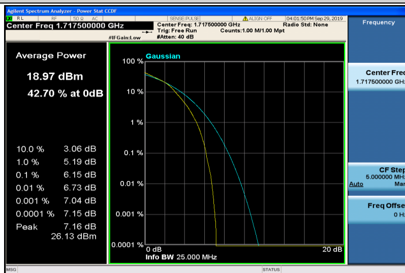
Band4-15MHz-16QAM-20025-75RB#0
