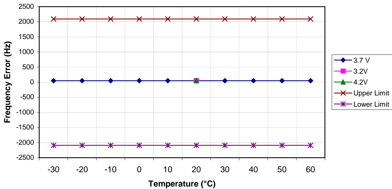
OVFKWC-KX5-5X0 AMPS 800 MHz Transmit RF Carrier Stability Over Temperature and Voltage
