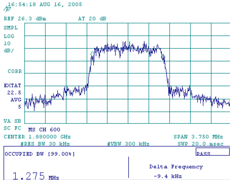
Figure 7-9 CDMA 1900 @ CH 600
