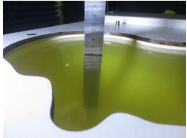
Fig. 9.2 Photo of Liquid Height for Head SAR (1710MHz~1910MHz) (depth>15cm)
