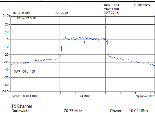
802.11ac (VHT80)_Chain 1 / CH138 (U-NII-2C Band)
