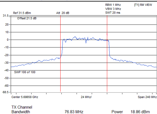
802.11ac (VHT80)_Chain 0 / CH138 (U-NII-2C Band)
