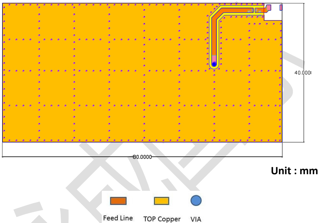
Evaluation Board Dimension
