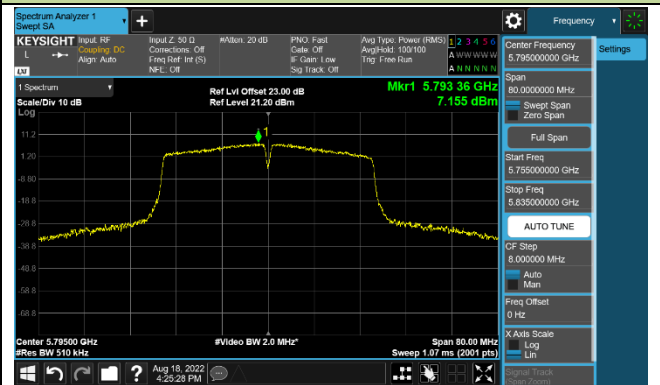
802.11ac-VHT80 Power Spectral Density - Ant 2
